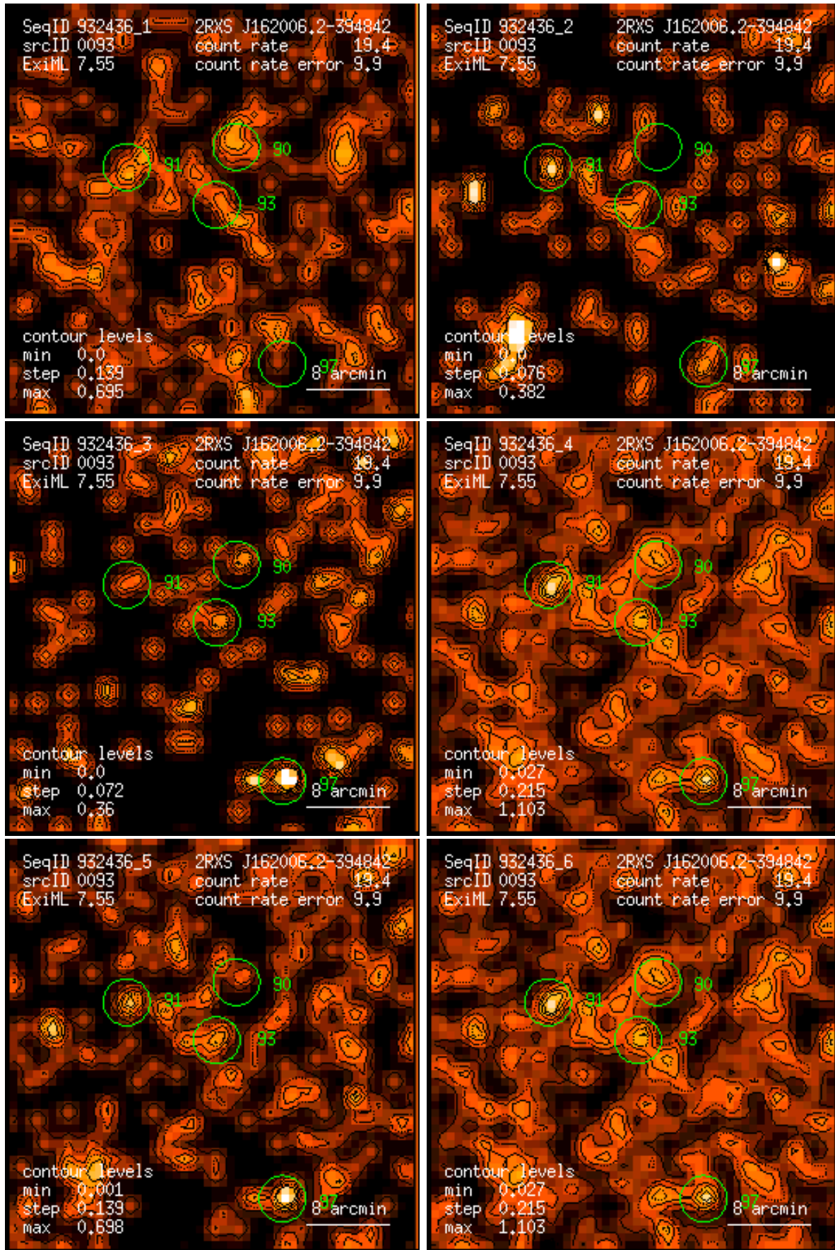
Figure 93: RASS 932436: detection 0093: band rate images, Gaussian filter: (1) PSPC channels 11 – 41, (2) 52 – 90, (3) 91 – 201, (4) 11 – 235, (5) 52 – 201, (6) 11 – 201. Broad band rates in counts/ks. Band rate contour levels in counts/ks/arcmin 2 .
