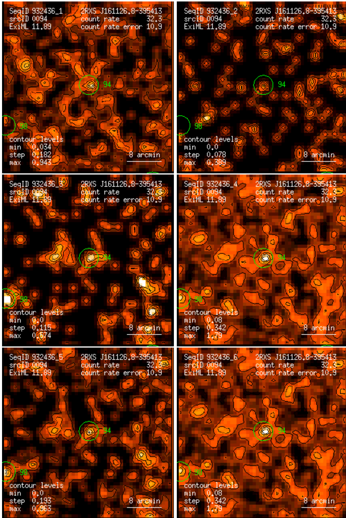
Figure 94: RASS 932436: detection 0094: band rate images, Gaussian filter: (1) PSPC channels 11 – 41, (2) 52 – 90, (3) 91 – 201, (4) 11 – 235, (5) 52 – 201, (6) 11 – 201. Broad band rates in counts/ks. Band rate contour levels in counts/ks/arcmin 2 .
