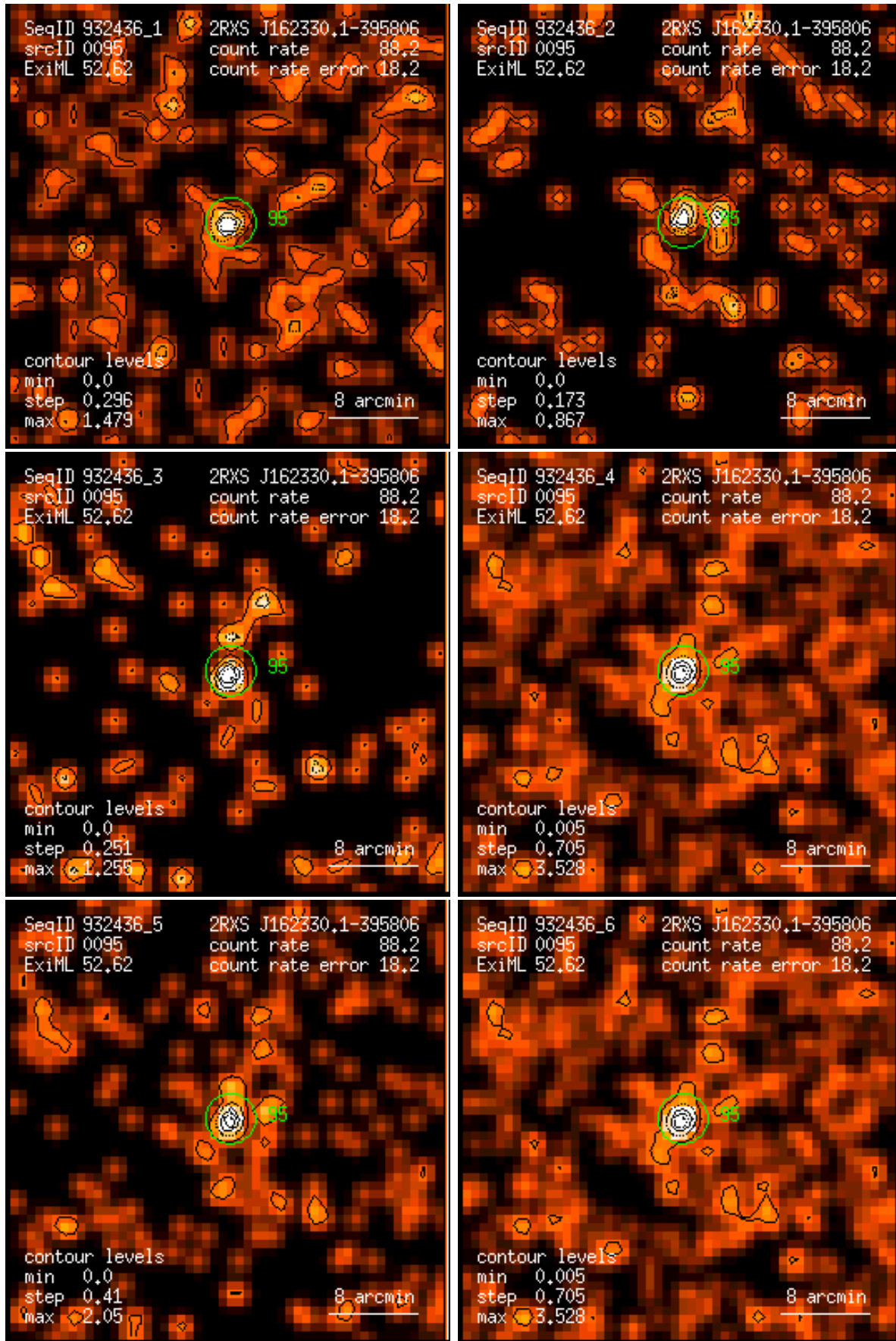
Figure 95: RASS 932436: detection 0095: band rate images, Gaussian filter: (1) PSPC channels 11 – 41, (2) 52 – 90, (3) 91 – 201, (4) 11 – 235, (5) 52 – 201, (6) 11 – 201. Broad band rates in counts/ks. Band rate contour levels in counts/ks/arcmin 2 .
