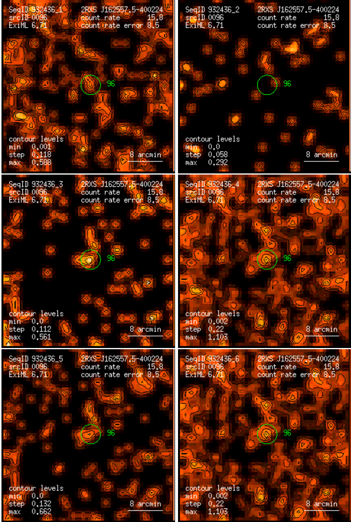
Figure 96: RASS 932436: detection 0096: band rate images, Gaussian filter: (1) PSPC channels 11 – 41, (2) 52 – 90, (3) 91 – 201, (4) 11 – 235, (5) 52 – 201, (6) 11 – 201. Broad band rates in counts/ks. Band rate contour levels in counts/ks/arcmin 2 .
