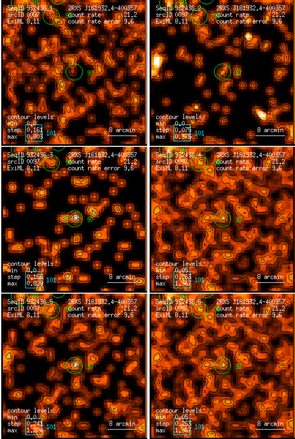
Figure 97: RASS 932436: detection 0097: band rate images, Gaussian filter: (1) PSPC channels 11 – 41, (2) 52 – 90, (3) 91 – 201, (4) 11 – 235, (5) 52 – 201, (6) 11 – 201. Broad band rates in counts/ks. Band rate contour levels in counts/ks/arcmin 2 .
