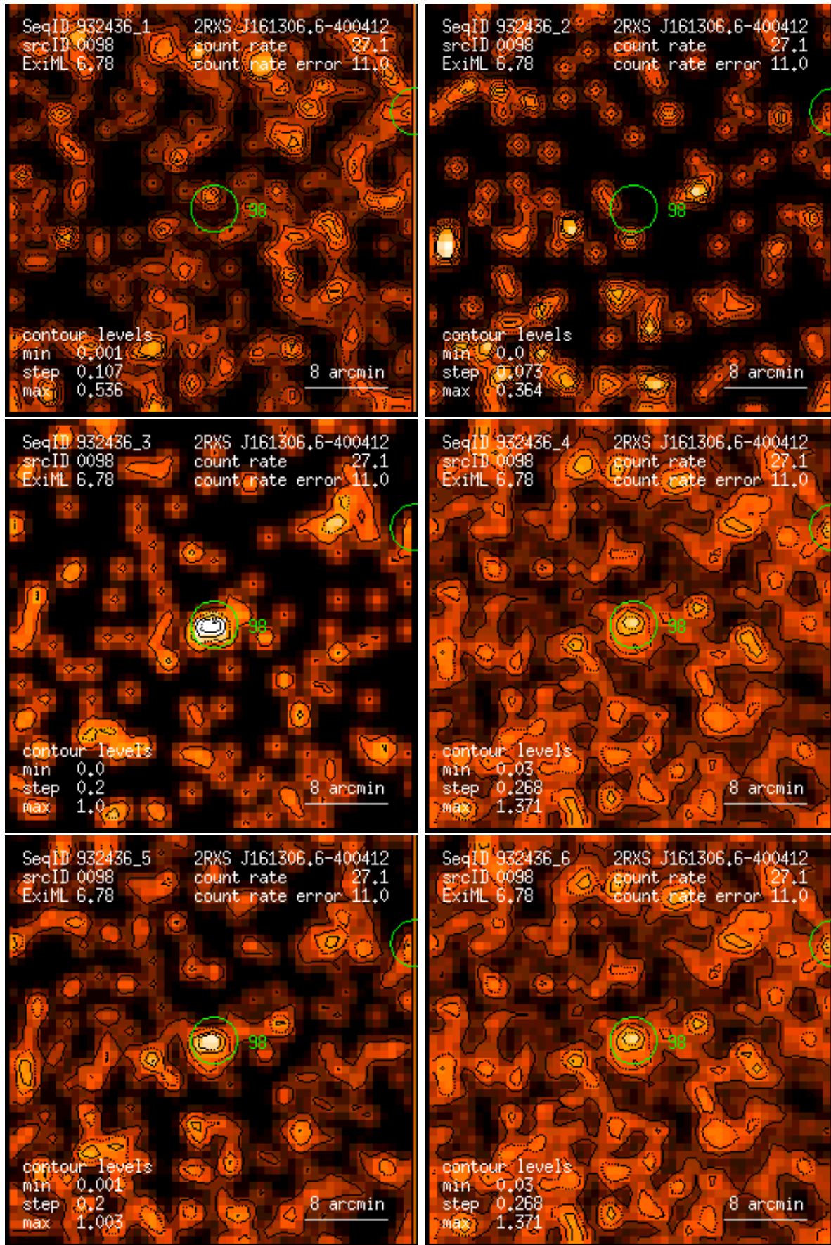
Figure 98: RASS 932436: detection 0098: band rate images, Gaussian filter: (1) PSPC channels 11 – 41, (2) 52 – 90, (3) 91 – 201, (4) 11 – 235, (5) 52 – 201, (6) 11 – 201. Broad band rates in counts/ks. Band rate contour levels in counts/ks/arcmin 2 .
