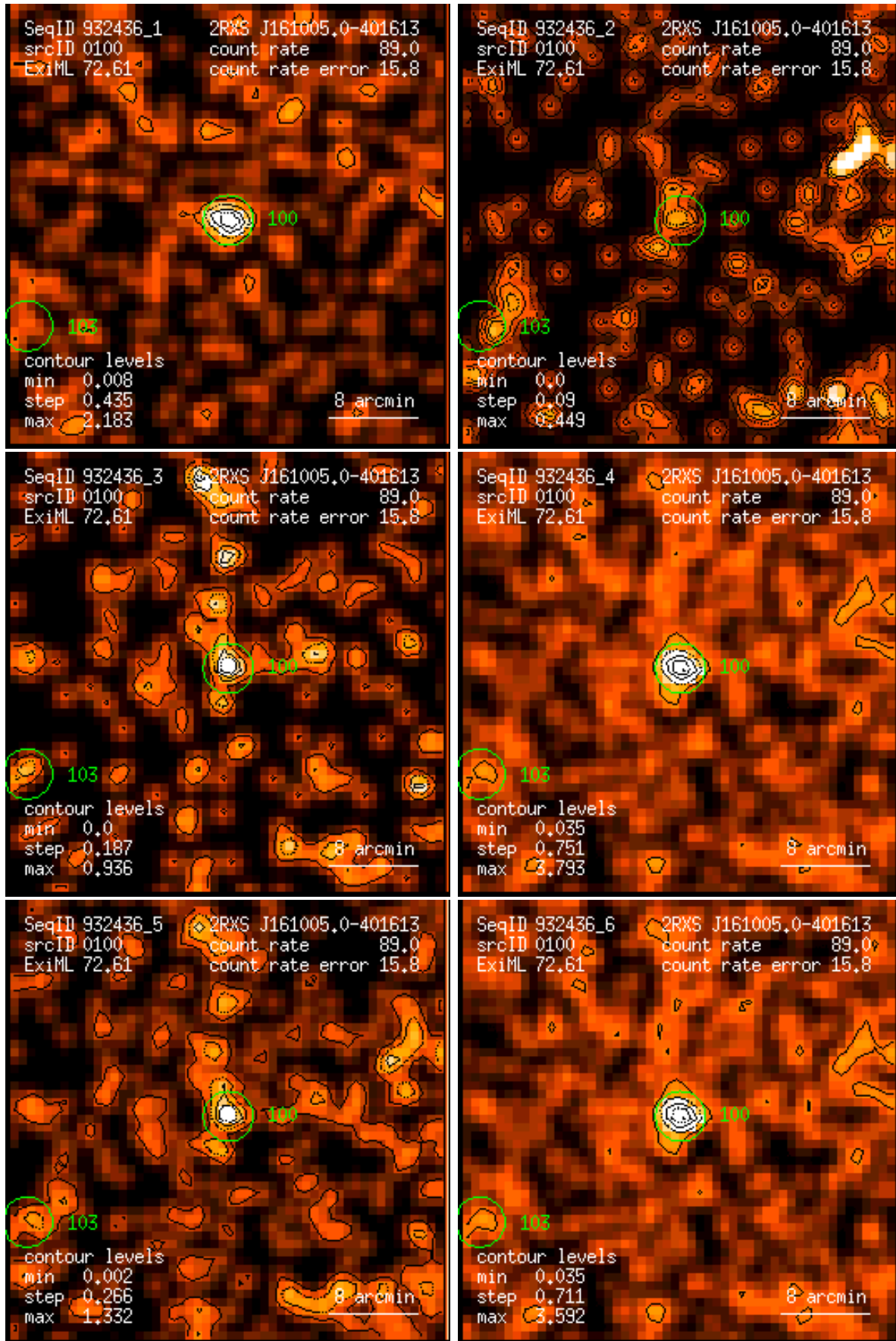
Figure 100: RASS 932436: detection 0100: band rate images, Gaussian filter: (1) PSPC channels 11 – 41, (2) 52 – 90, (3) 91 – 201, (4) 11 – 235, (5) 52 – 201, (6) 11 – 201. Broad band rates in counts/ks. Band rate contour levels in counts/ks/arcmin 2 .
