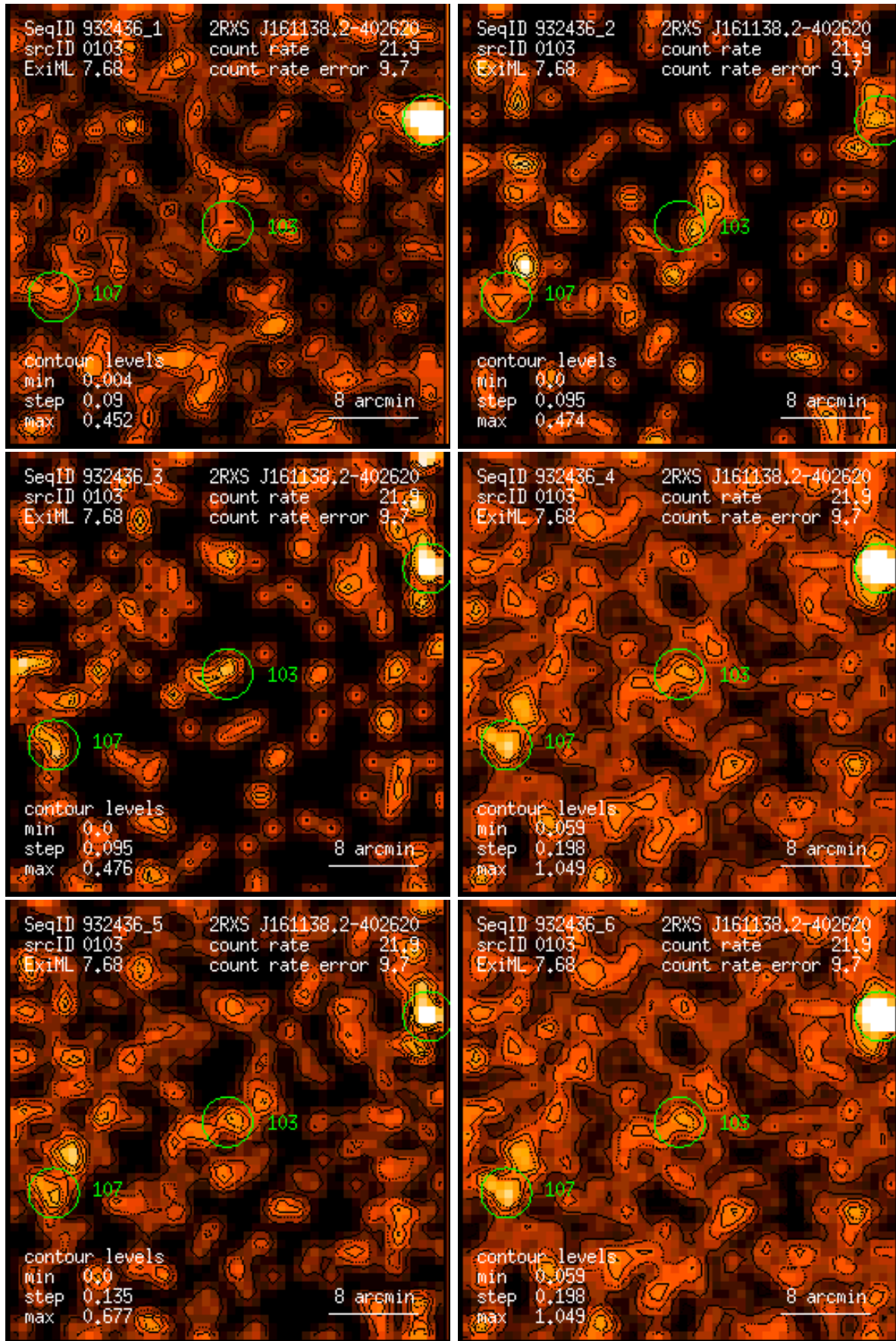
Figure 103: RASS 932436: detection 0103: band rate images, Gaussian filter: (1) PSPC channels 11 – 41, (2) 52 – 90, (3) 91 – 201, (4) 11 – 235, (5) 52 – 201, (6) 11 – 201. Broad band rates in counts/ks. Band rate contour levels in counts/ks/arcmin 2 .
