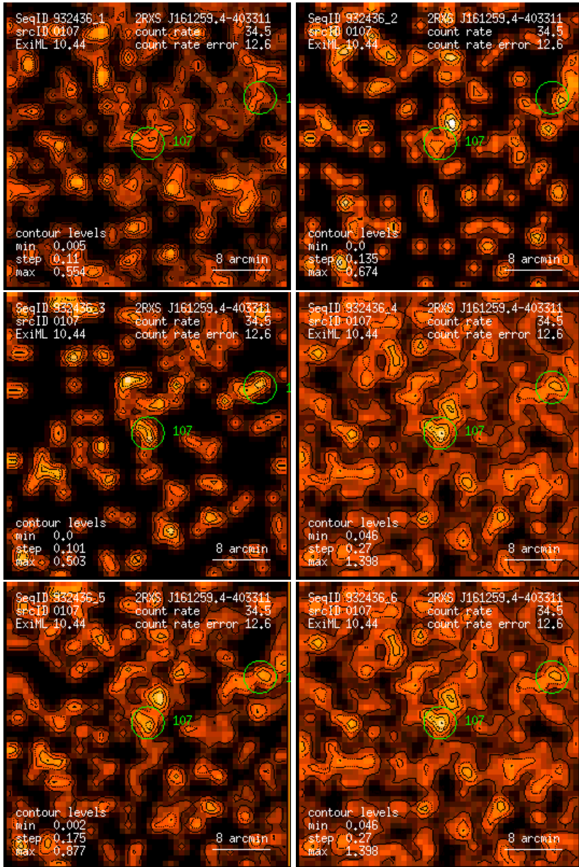
Figure 107: RASS 932436: detection 0107: band rate images, Gaussian filter: (1) PSPC channels 11 – 41, (2) 52 – 90, (3) 91 – 201, (4) 11 – 235, (5) 52 – 201, (6) 11 – 201. Broad band rates in counts/ks. Band rate contour levels in counts/ks/arcmin 2 .
