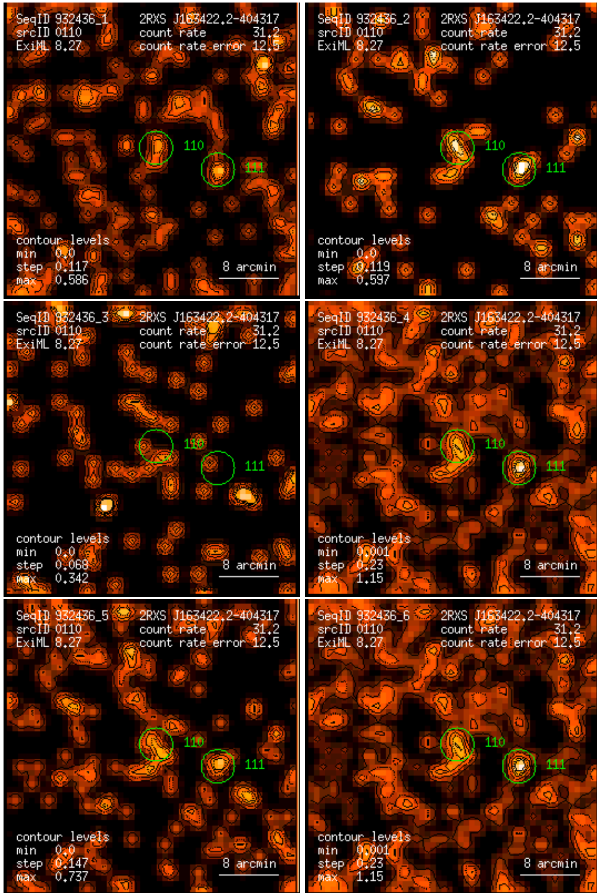
Figure 110: RASS 932436: detection 0110: band rate images, Gaussian filter: (1) PSPC channels 11 – 41, (2) 52 – 90, (3) 91 – 201, (4) 11 – 235, (5) 52 – 201, (6) 11 – 201. Broad band rates in counts/ks. Band rate contour levels in counts/ks/arcmin 2 .
