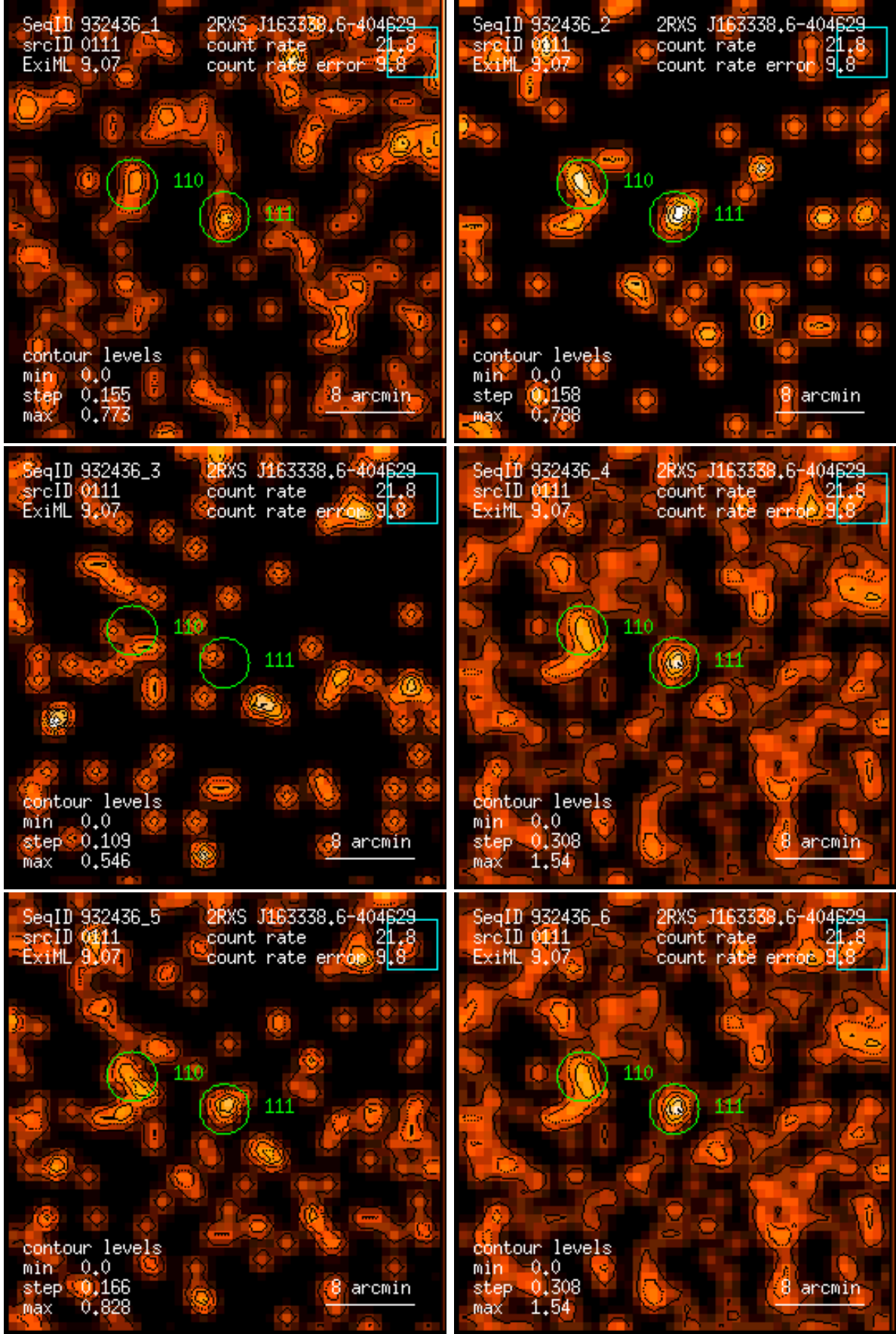
Figure 111: RASS 932436: detection 0111: band rate images, Gaussian filter: (1) PSPC channels 11 – 41, (2) 52 – 90, (3) 91 – 201, (4) 11 – 235, (5) 52 – 201, (6) 11 – 201. Broad band rates in counts/ks. Band rate contour levels in counts/ks/arcmin 2 .
