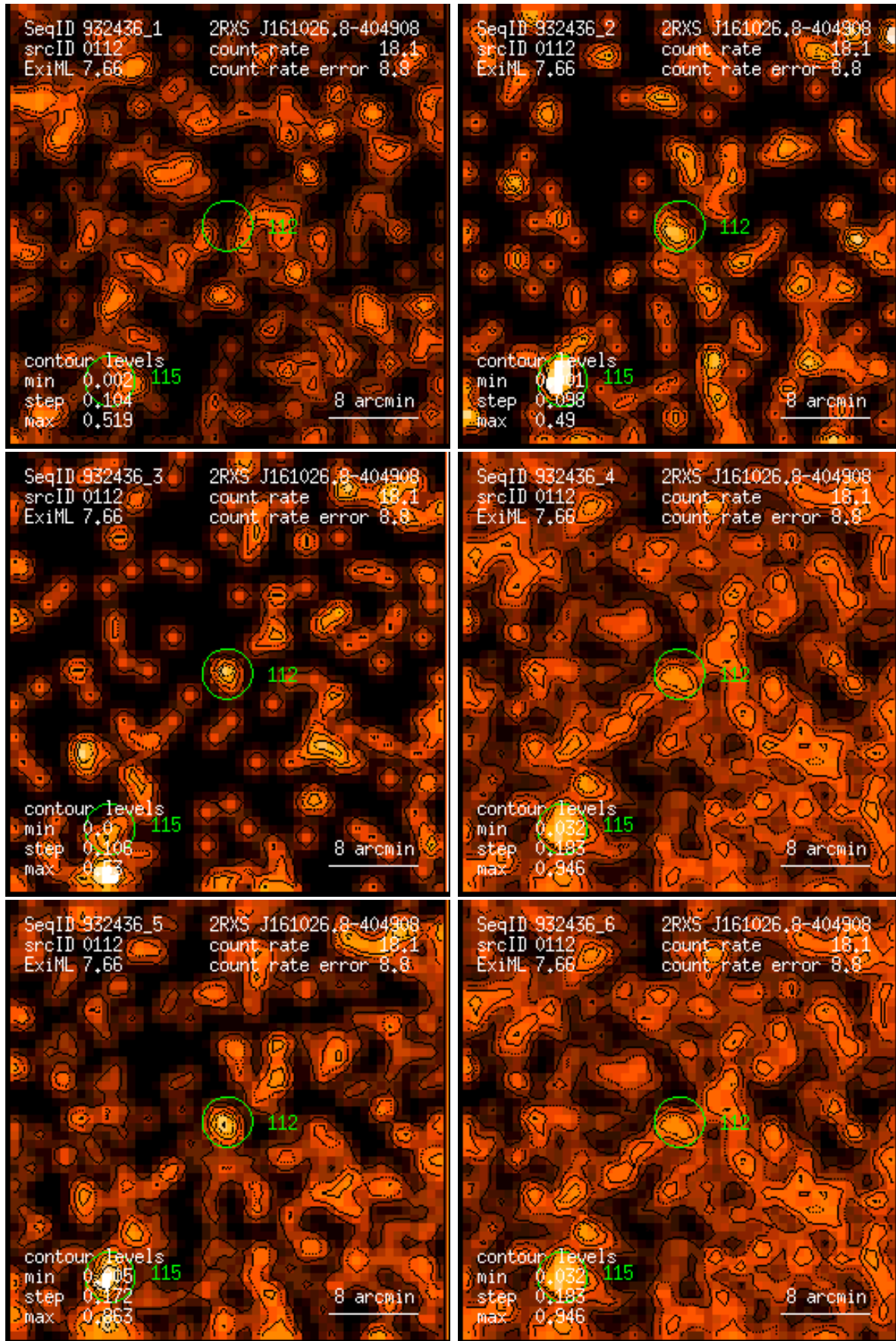
Figure 112: RASS 932436: detection 0112: band rate images, Gaussian filter: (1) PSPC channels 11 – 41, (2) 52 – 90, (3) 91 – 201, (4) 11 – 235, (5) 52 – 201, (6) 11 – 201. Broad band rates in counts/ks. Band rate contour levels in counts/ks/arcmin 2 .
