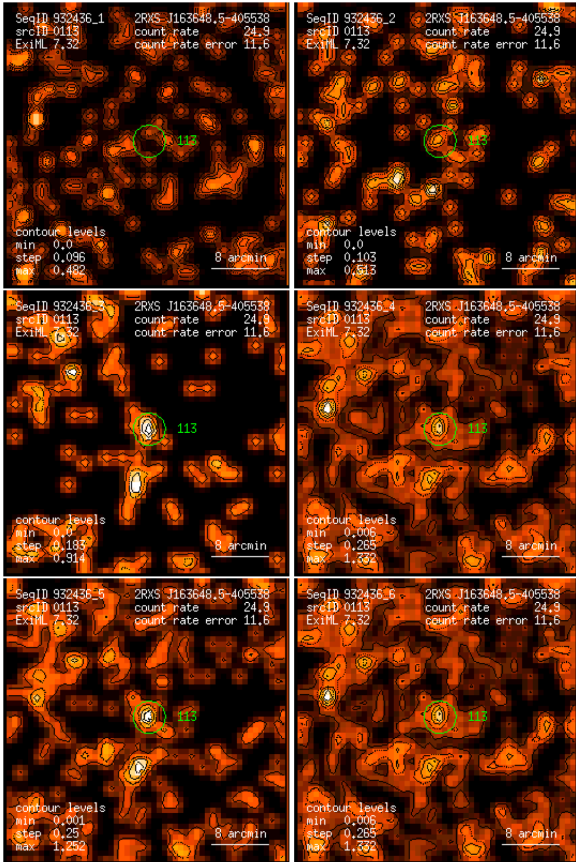
Figure 113: RASS 932436: detection 0113: band rate images, Gaussian filter: (1) PSPC channels 11 – 41, (2) 52 – 90, (3) 91 – 201, (4) 11 – 235, (5) 52 – 201, (6) 11 – 201. Broad band rates in counts/ks. Band rate contour levels in counts/ks/arcmin 2 .
