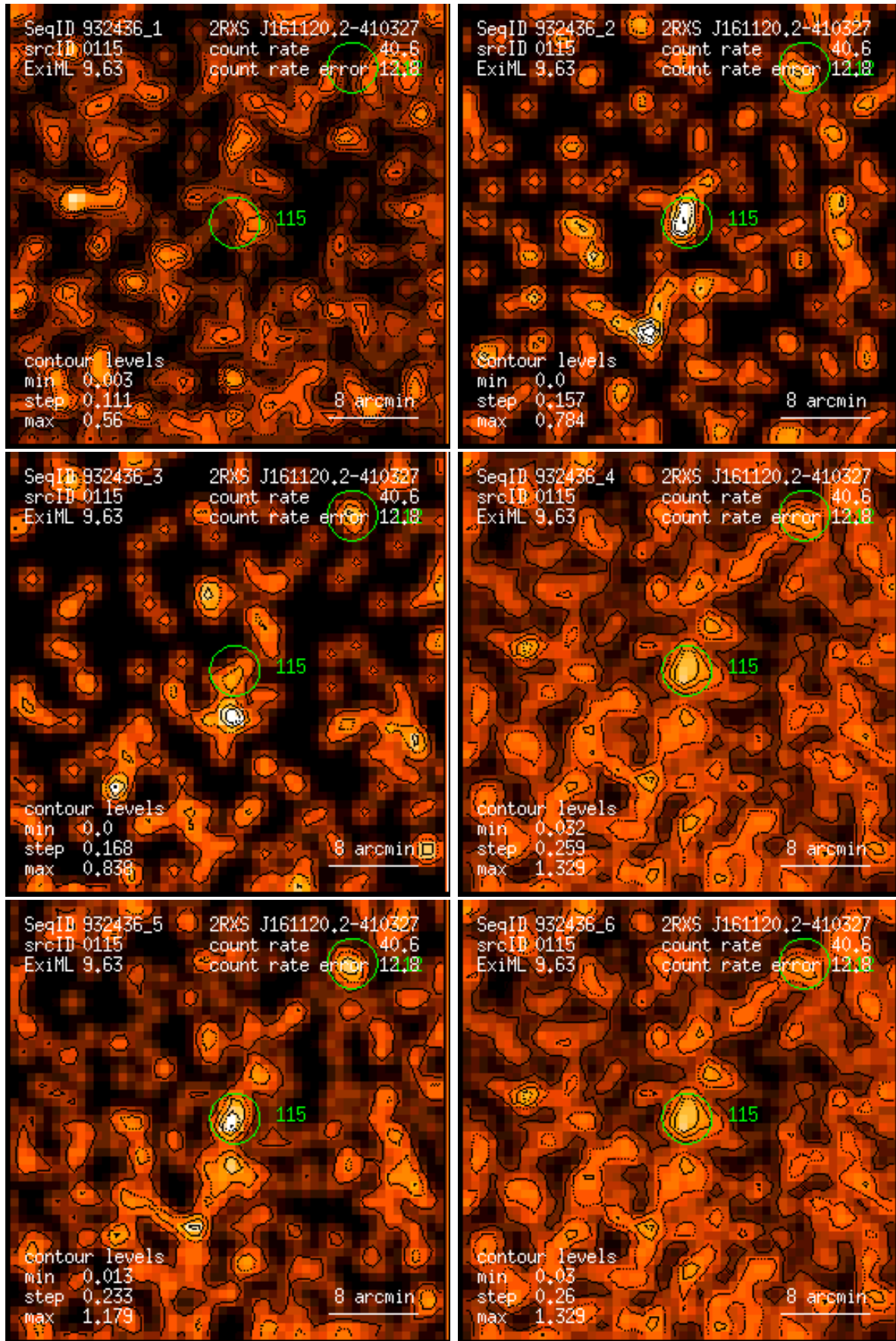
Figure 115: RASS 932436: detection 0115: band rate images, Gaussian filter: (1) PSPC channels 11 – 41, (2) 52 – 90, (3) 91 – 201, (4) 11 – 235, (5) 52 – 201, (6) 11 – 201. Broad band rates in counts/ks. Band rate contour levels in counts/ks/arcmin 2 .
