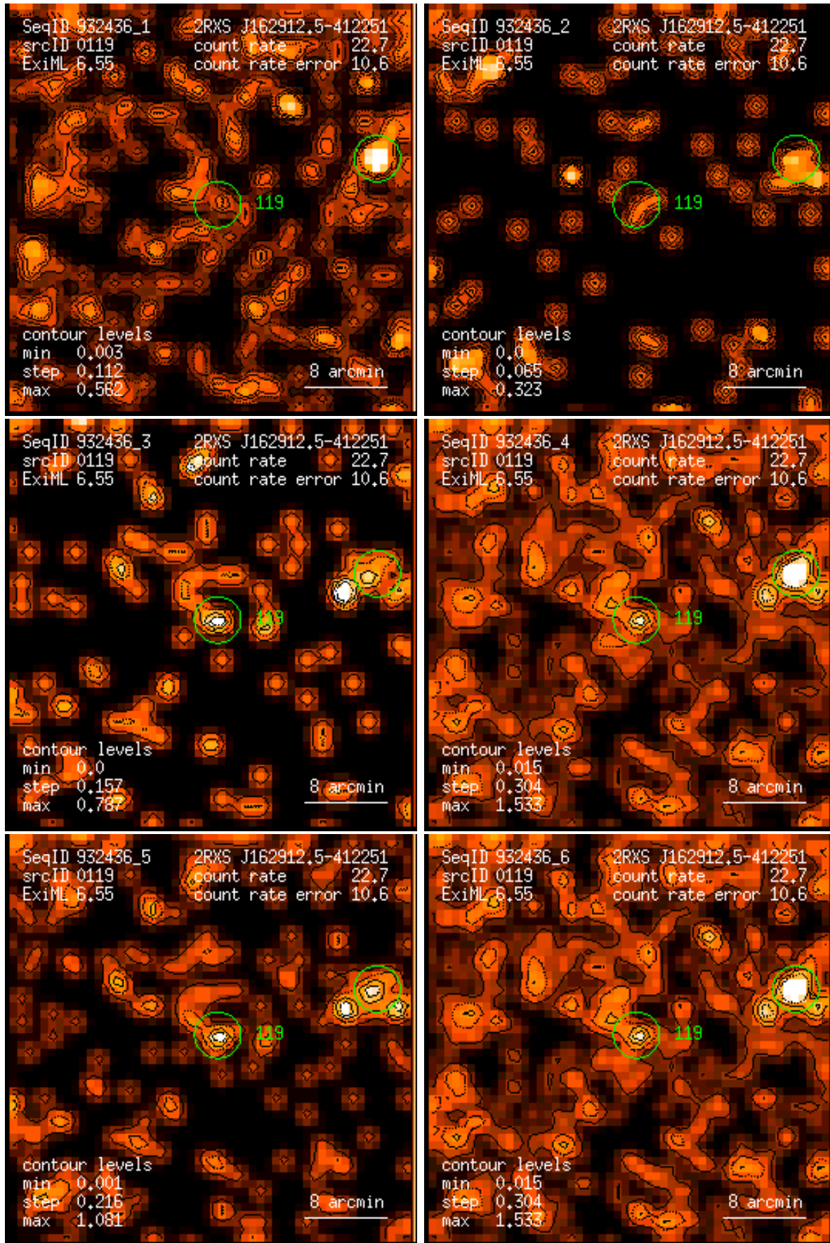
Figure 119: RASS 932436: detection 0119: band rate images, Gaussian filter: (1) PSPC channels 11 – 41, (2) 52 – 90, (3) 91 – 201, (4) 11 – 235, (5) 52 – 201, (6) 11 – 201. Broad band rates in counts/ks. Band rate contour levels in counts/ks/arcmin 2 .
