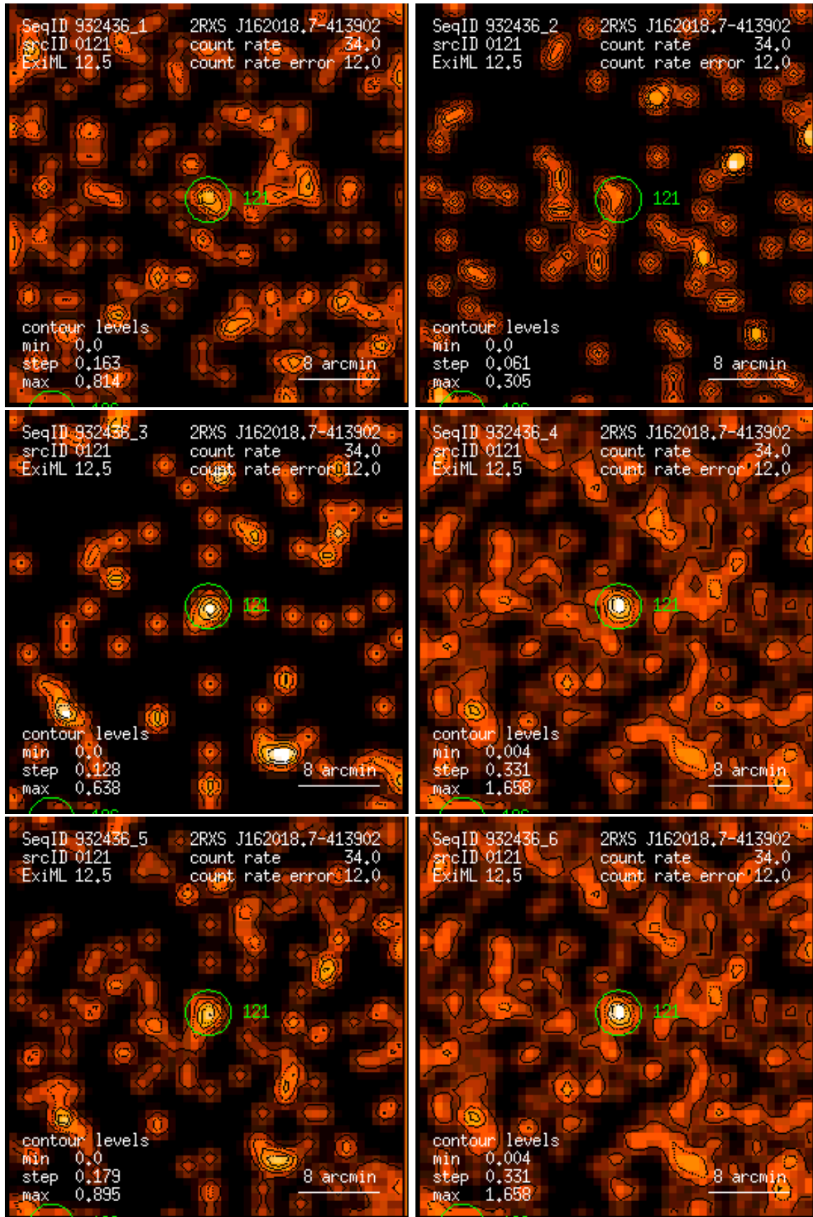
Figure 121: RASS 932436: detection 0121: band rate images, Gaussian filter: (1) PSPC channels 11 – 41, (2) 52 – 90, (3) 91 – 201, (4) 11 – 235, (5) 52 – 201, (6) 11 – 201. Broad band rates in counts/ks. Band rate contour levels in counts/ks/arcmin 2 .
