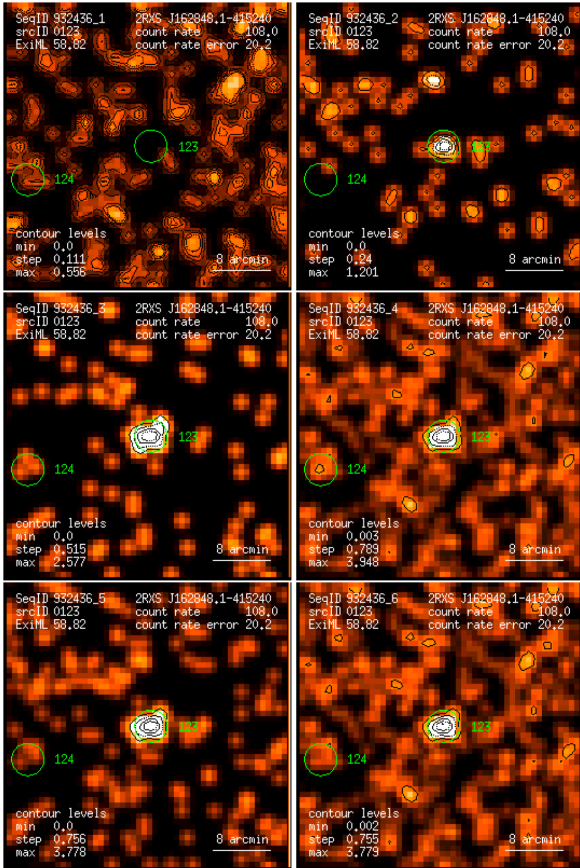
Figure 123: RASS 932436: detection 0123: band rate images, Gaussian filter: (1) PSPC channels 11 – 41, (2) 52 – 90, (3) 91 – 201, (4) 11 – 235, (5) 52 – 201, (6) 11 – 201. Broad band rates in counts/ks. Band rate contour levels in counts/ks/arcmin 2 .
