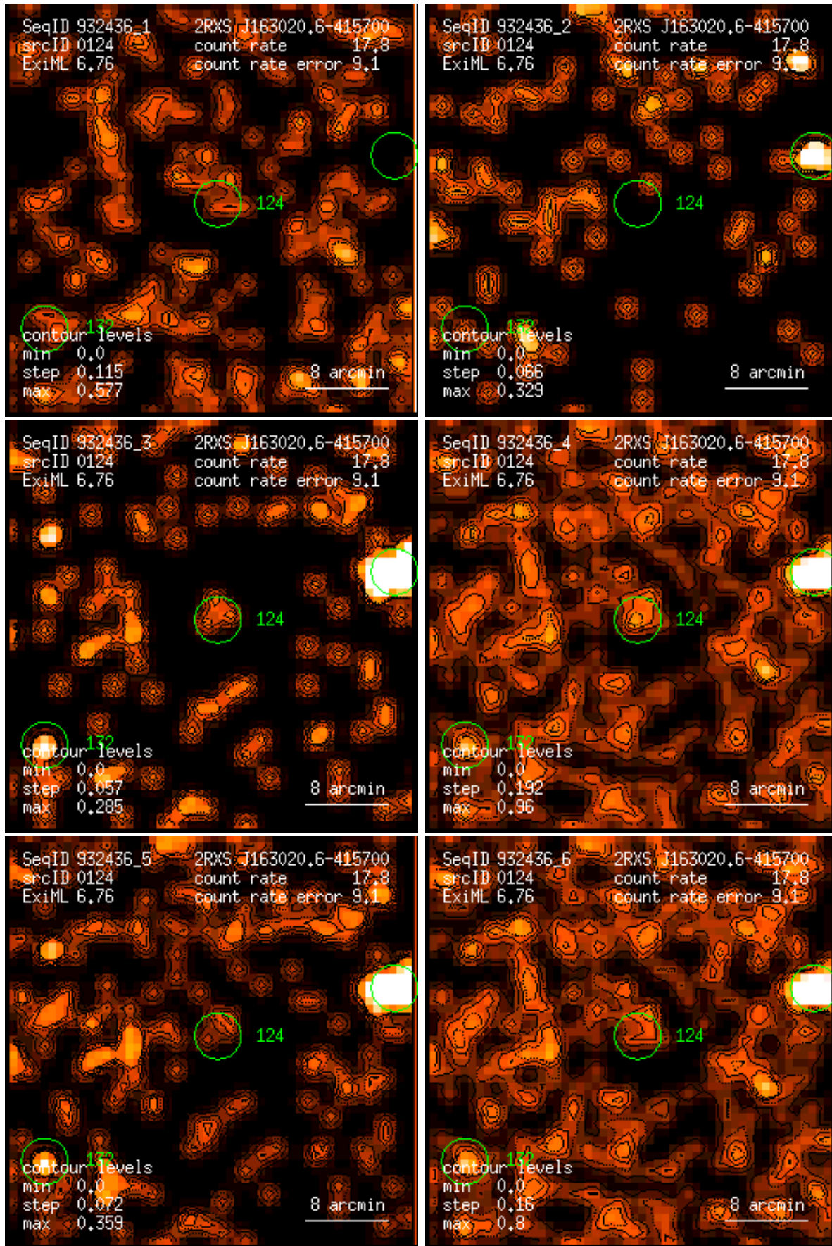
Figure 124: RASS 932436: detection 0124: band rate images, Gaussian filter: (1) PSPC channels 11 – 41, (2) 52 – 90, (3) 91 – 201, (4) 11 – 235, (5) 52 – 201, (6) 11 – 201. Broad band rates in counts/ks. Band rate contour levels in counts/ks/arcmin 2 .
