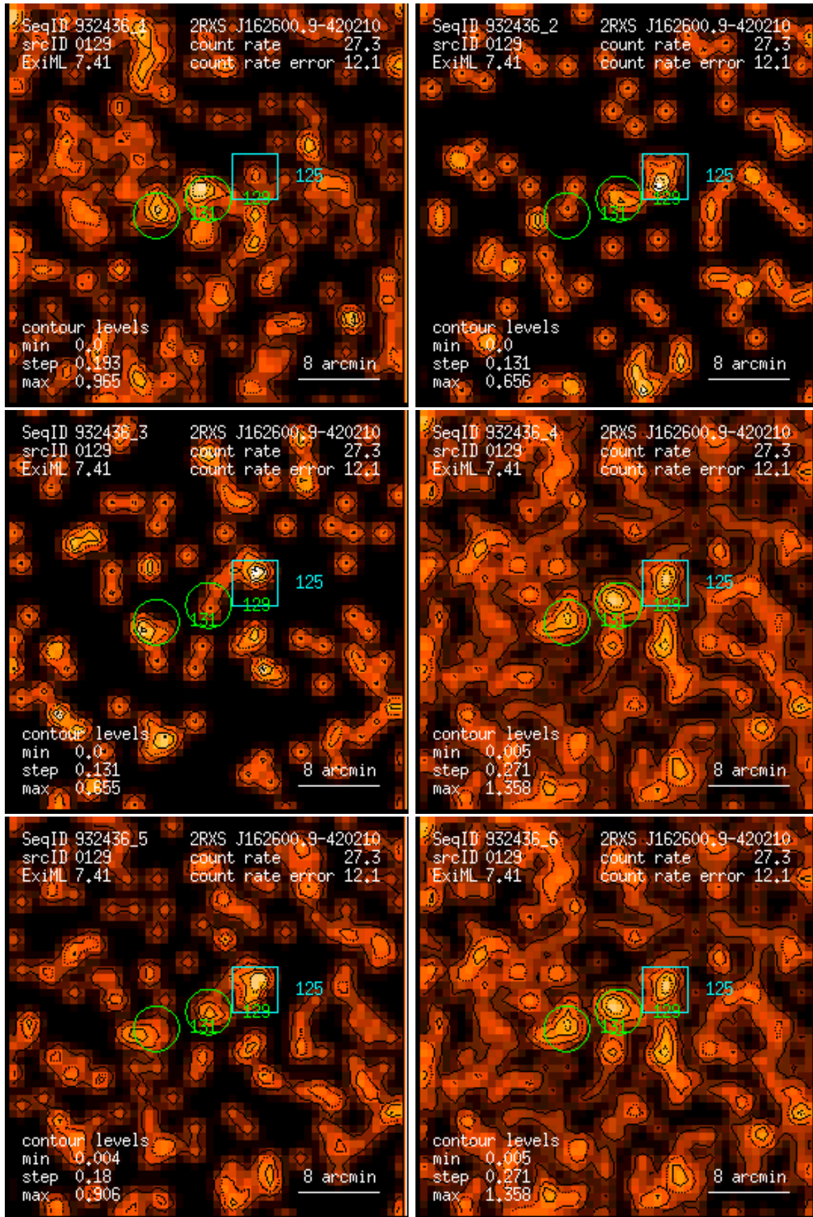
Figure 129: RASS 932436: detection 0129: band rate images, Gaussian filter: (1) PSPC channels 11 – 41, (2) 52 – 90, (3) 91 – 201, (4) 11 – 235, (5) 52 – 201, (6) 11 – 201. Broad band rates in counts/ks. Band rate contour levels in counts/ks/arcmin 2 .
