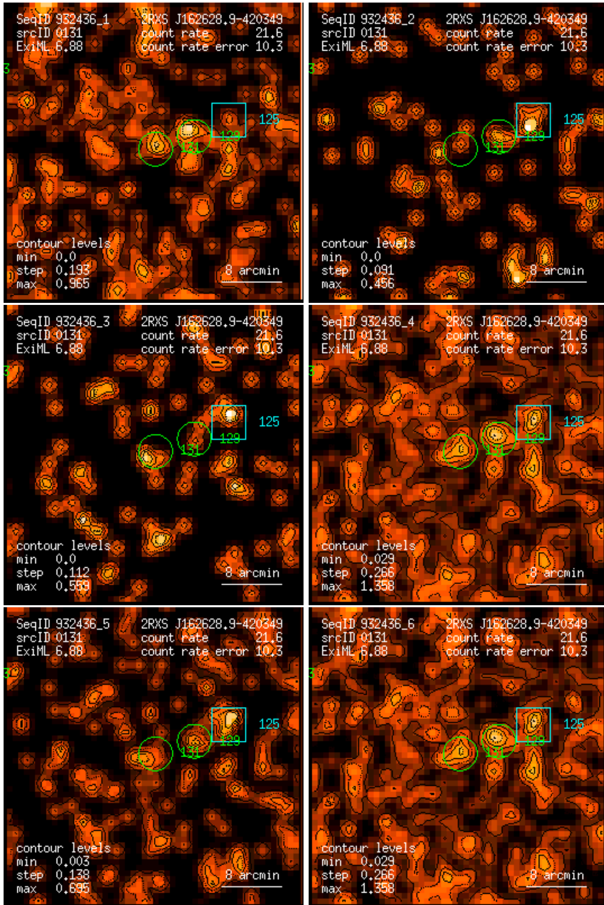
Figure 131: RASS 932436: detection 0131: band rate images, Gaussian filter: (1) PSPC channels 11 – 41, (2) 52 – 90, (3) 91 – 201, (4) 11 – 235, (5) 52 – 201, (6) 11 – 201. Broad band rates in counts/ks. Band rate contour levels in counts/ks/arcmin 2 .
