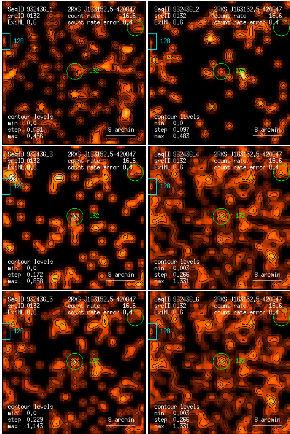
Figure 132: RASS 932436: detection 0132: band rate images, Gaussian filter: (1) PSPC channels 11 – 41, (2) 52 – 90, (3) 91 – 201, (4) 11 – 235, (5) 52 – 201, (6) 11 – 201. Broad band rates in counts/ks. Band rate contour levels in counts/ks/arcmin 2 .
