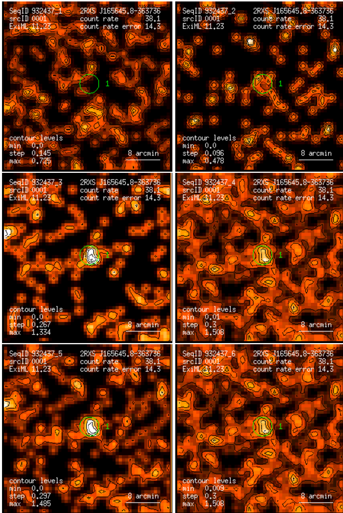
Figure 1: RASS 932437: detection 0001: band rate images, Gaussian filter: (1) PSPC channels 11 – 41, (2) 52 – 90, (3) 91 – 201, (4) 11 – 235, (5) 52 – 201, (6) 11 – 201. Broad band rates in counts/ks. Band rate contour levels in counts/ks/arcmin 2 .
