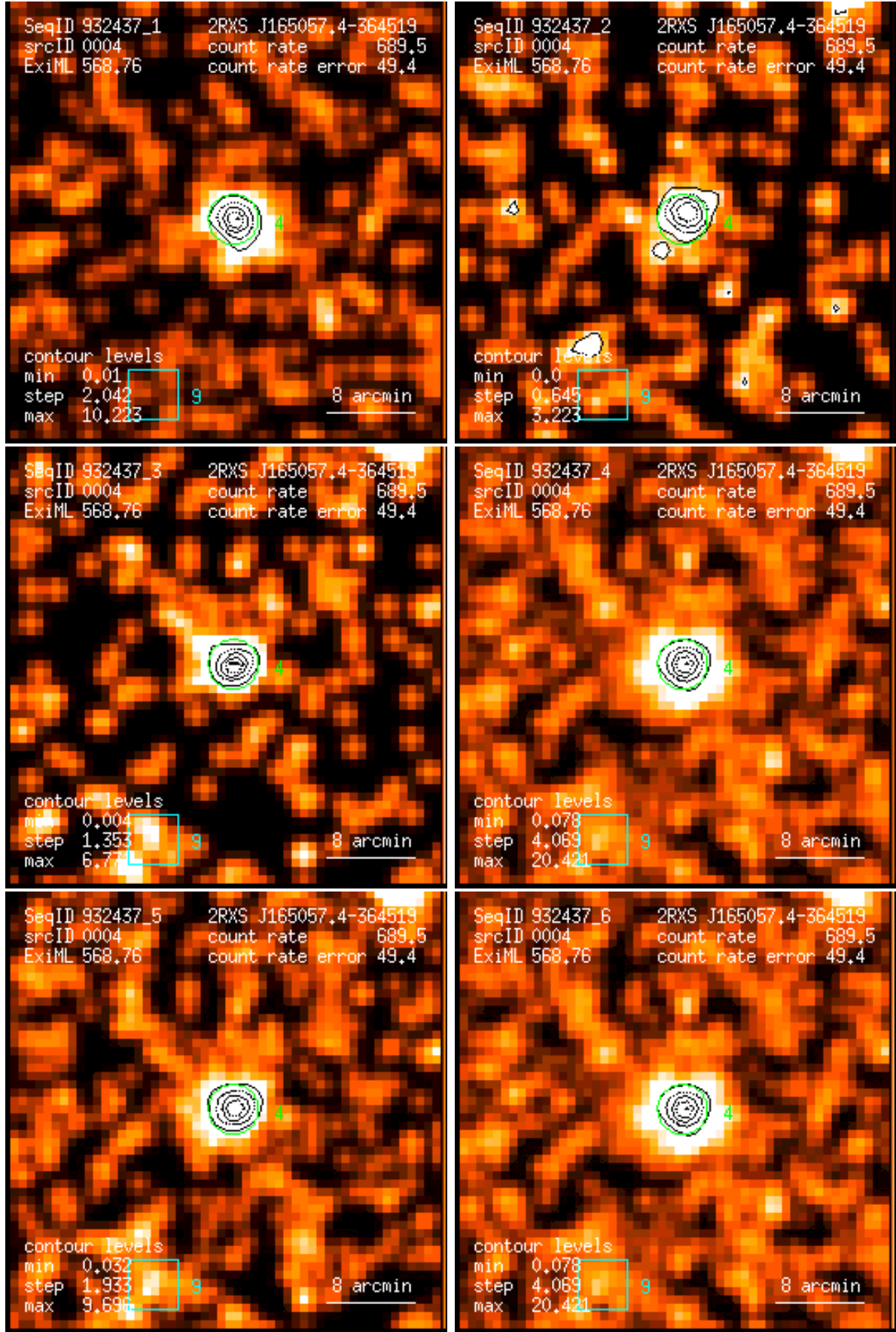
Figure 4: RASS 932437: detection 0004: band rate images, Gaussian filter: (1) PSPC channels 11 – 41, (2) 52 – 90, (3) 91 – 201, (4) 11 – 235, (5) 52 – 201, (6) 11 – 201. Broad band rates in counts/ks. Band rate contour levels in counts/ks/arcmin 2 .
