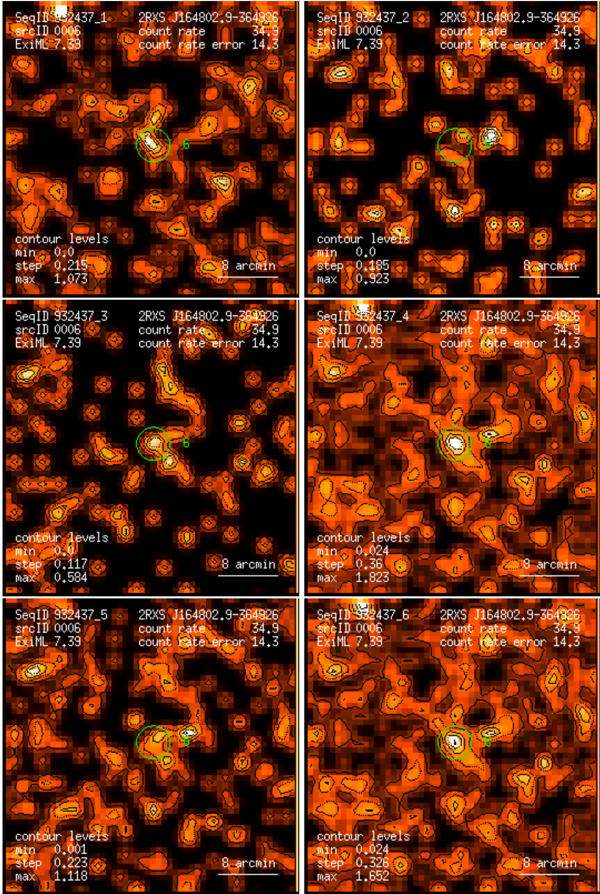
Figure 6: RASS 932437: detection 0006: band rate images, Gaussian filter: (1) PSPC channels 11 – 41, (2) 52 – 90, (3) 91 – 201, (4) 11 – 235, (5) 52 – 201, (6) 11 – 201. Broad band rates in counts/ks. Band rate contour levels in counts/ks/arcmin 2 .
