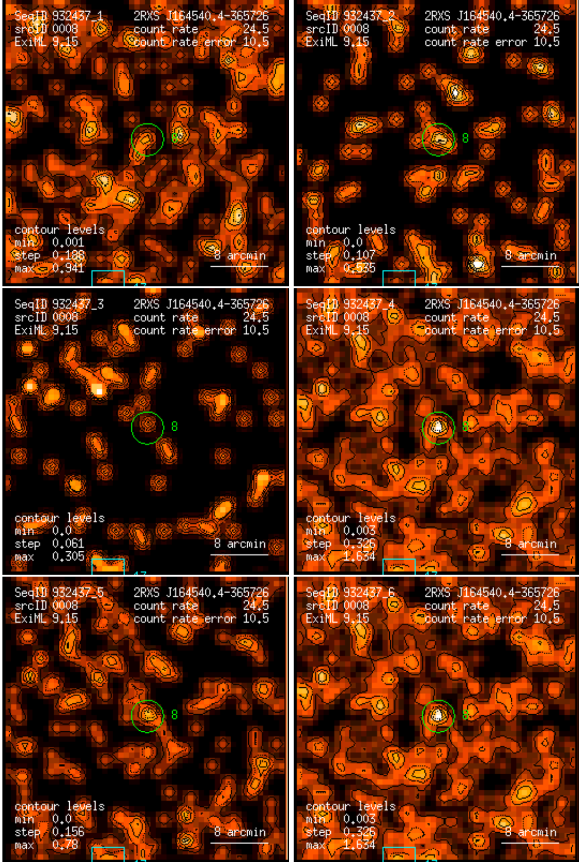
Figure 8: RASS 932437: detection 0008: band rate images, Gaussian filter: (1) PSPC channels 11 – 41, (2) 52 – 90, (3) 91 – 201, (4) 11 – 235, (5) 52 – 201, (6) 11 – 201. Broad band rates in counts/ks. Band rate contour levels in counts/ks/arcmin 2 .
