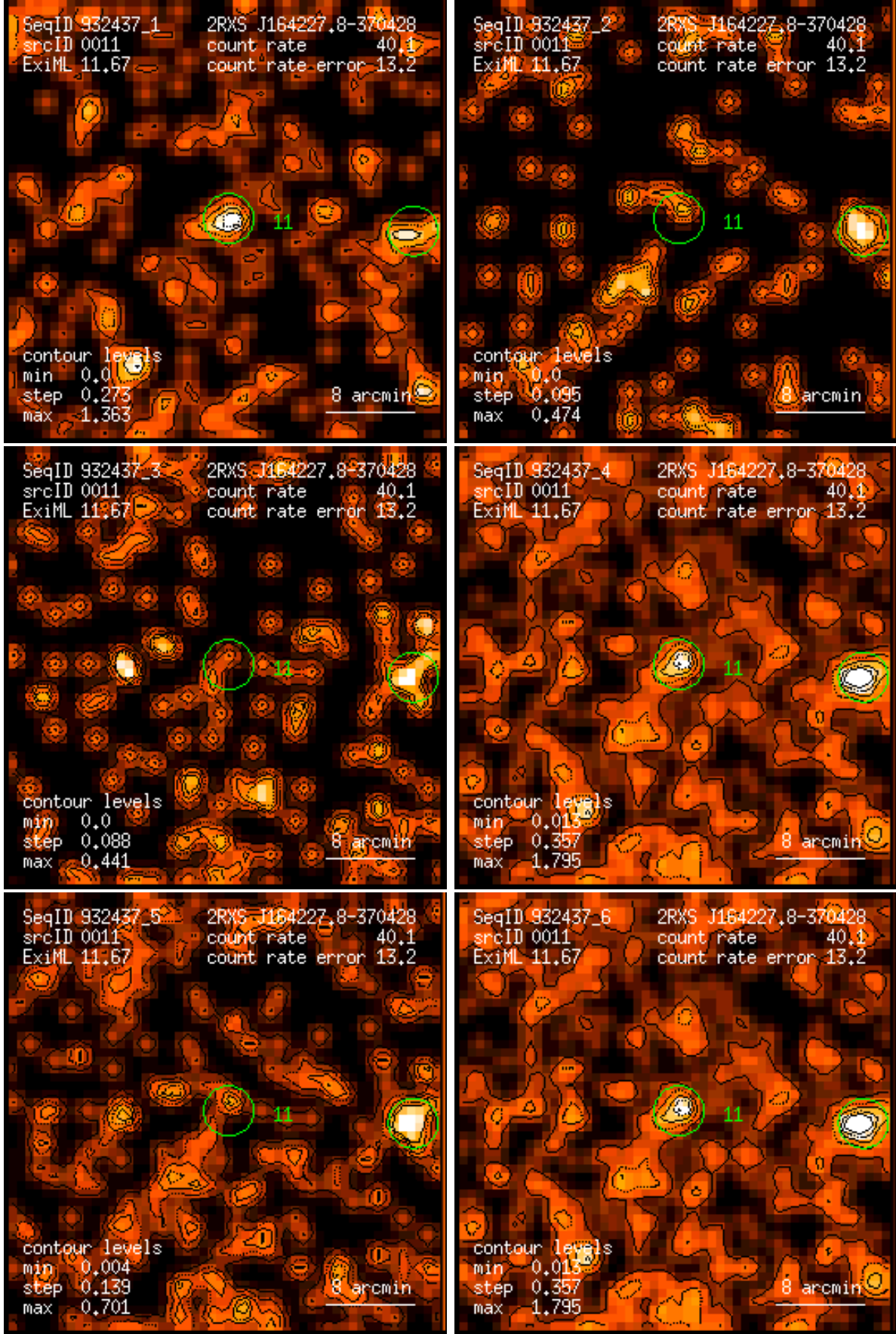
Figure 11: RASS 932437: detection 0011: band rate images, Gaussian filter: (1) PSPC channels 11 – 41, (2) 52 – 90, (3) 91 – 201, (4) 11 – 235, (5) 52 – 201, (6) 11 – 201. Broad band rates in counts/ks. Band rate contour levels in counts/ks/arcmin 2 .
