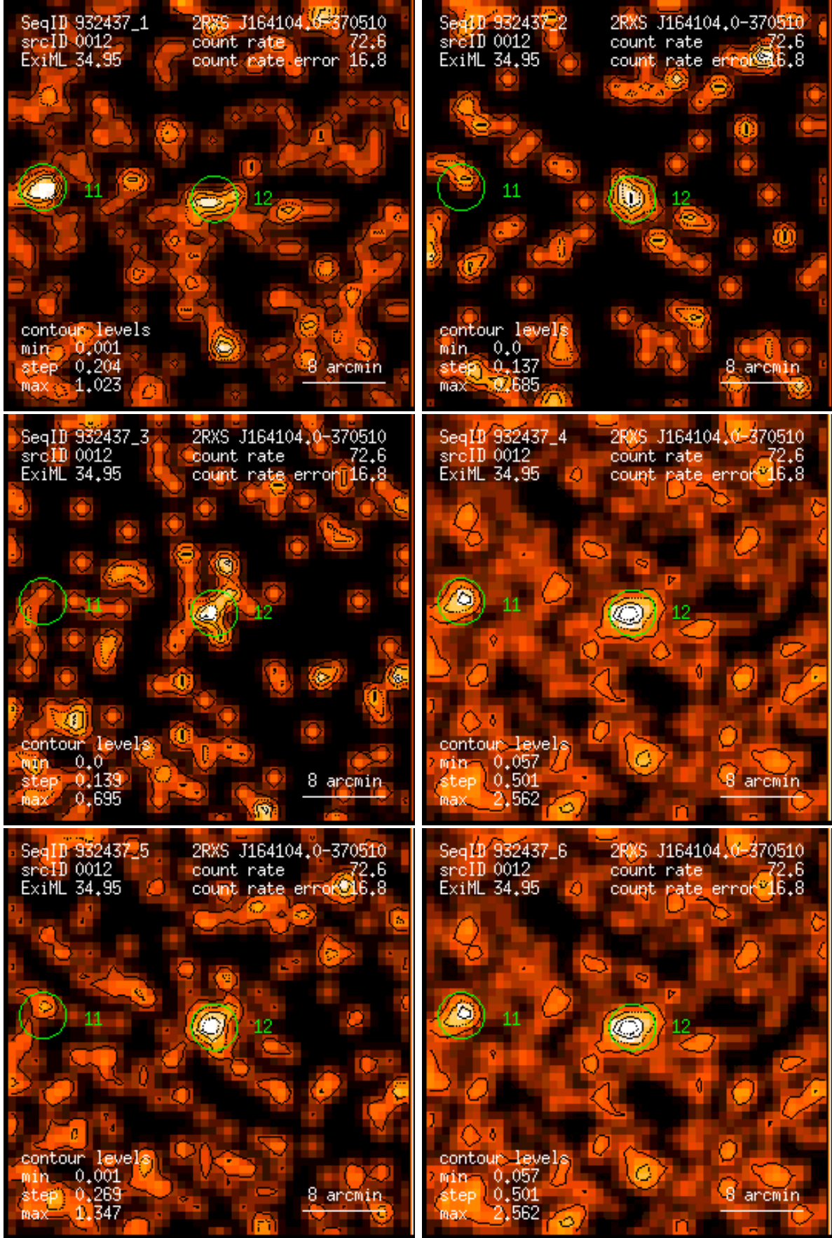
Figure 12: RASS 932437: detection 0012: band rate images, Gaussian filter: (1) PSPC channels 11 – 41, (2) 52 – 90, (3) 91 – 201, (4) 11 – 235, (5) 52 – 201, (6) 11 – 201. Broad band rates in counts/ks. Band rate contour levels in counts/ks/arcmin 2 .
