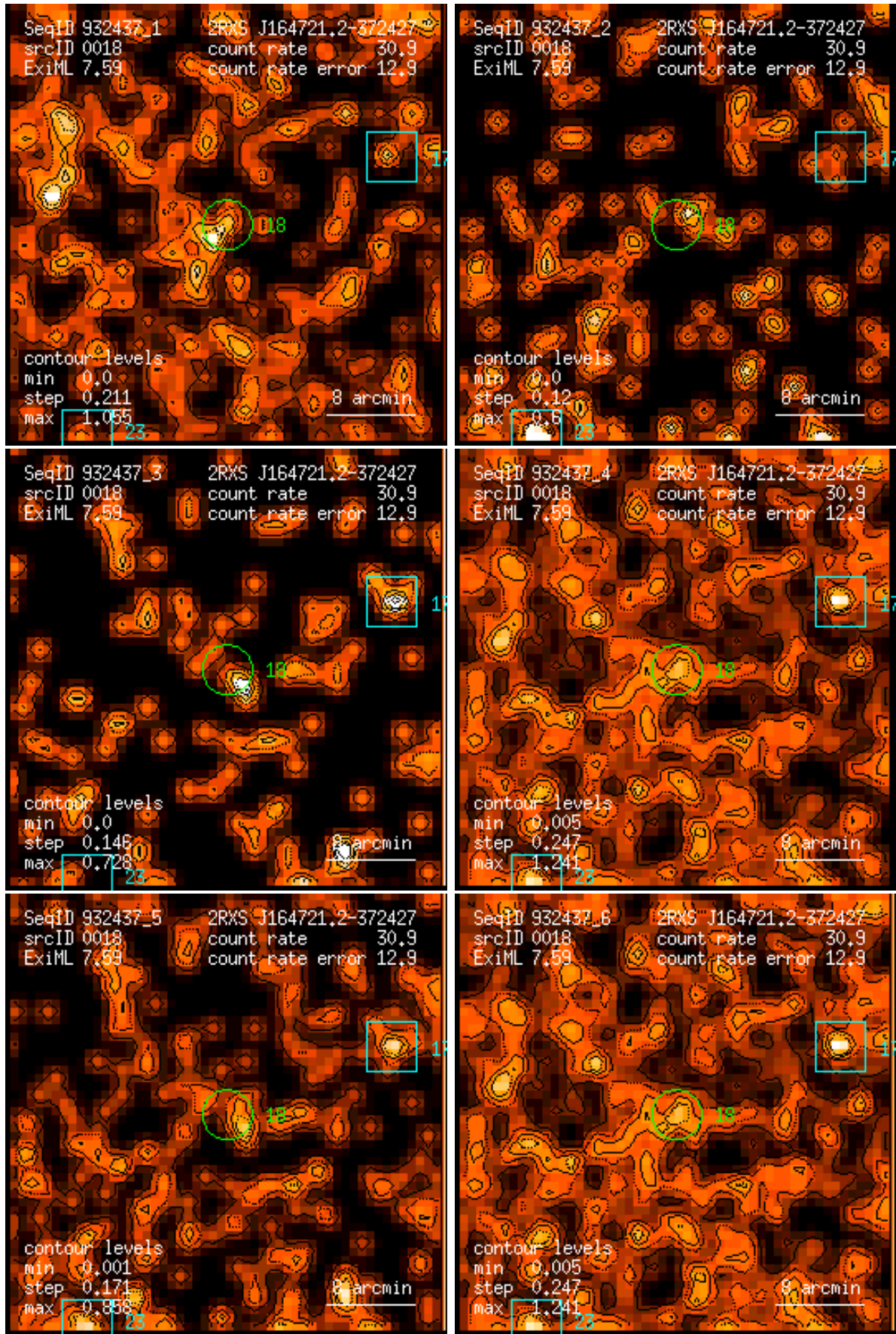
Figure 18: RASS 932437: detection 0018: band rate images, Gaussian filter: (1) PSPC channels 11 – 41, (2) 52 – 90, (3) 91 – 201, (4) 11 – 235, (5) 52 – 201, (6) 11 – 201. Broad band rates in counts/ks. Band rate contour levels in counts/ks/arcmin 2 .
