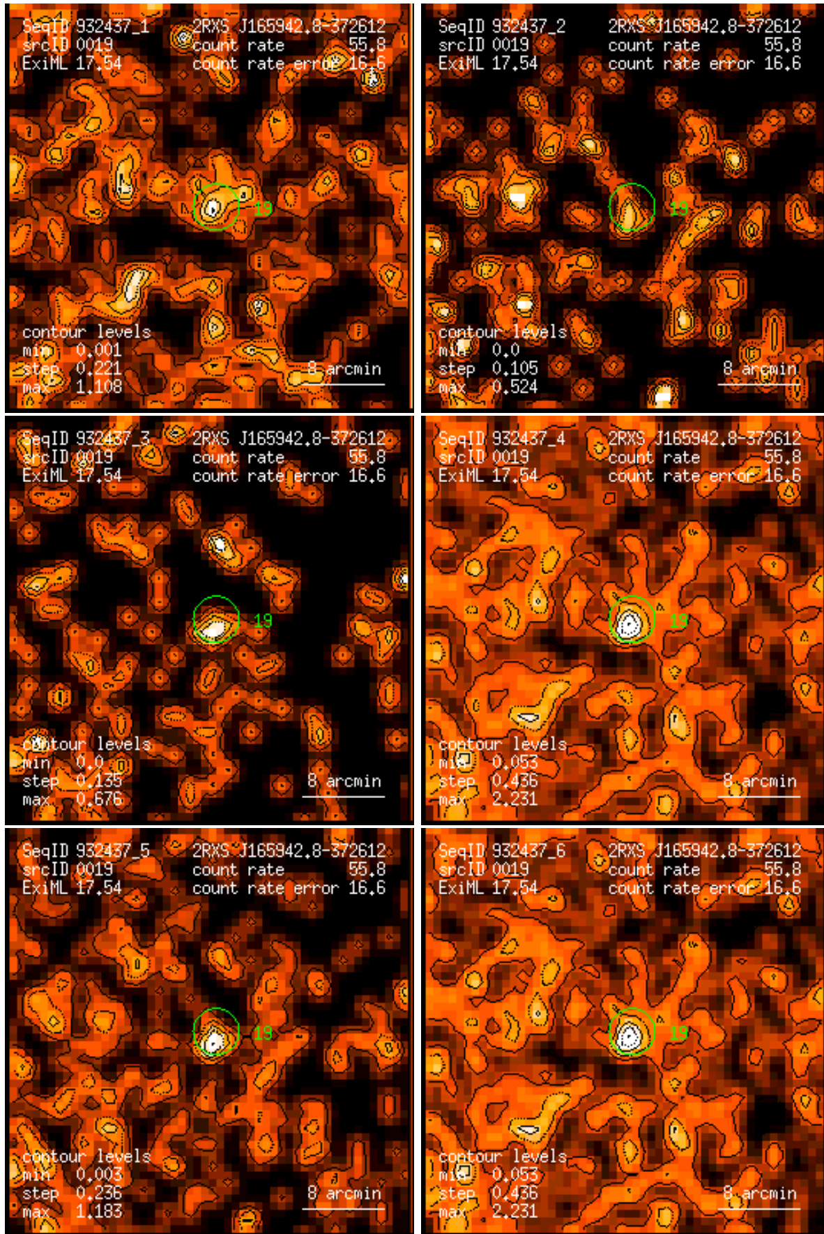
Figure 19: RASS 932437: detection 0019: band rate images, Gaussian filter: (1) PSPC channels 11 – 41, (2) 52 – 90, (3) 91 – 201, (4) 11 – 235, (5) 52 – 201, (6) 11 – 201. Broad band rates in counts/ks. Band rate contour levels in counts/ks/arcmin 2 .
