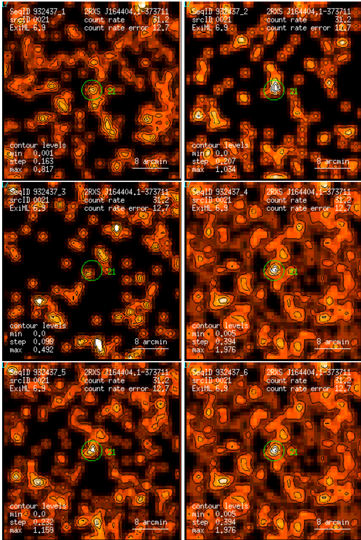
Figure 21: RASS 932437: detection 0021: band rate images, Gaussian filter: (1) PSPC channels 11 – 41, (2) 52 – 90, (3) 91 – 201, (4) 11 – 235, (5) 52 – 201, (6) 11 – 201. Broad band rates in counts/ks. Band rate contour levels in counts/ks/arcmin 2 .
