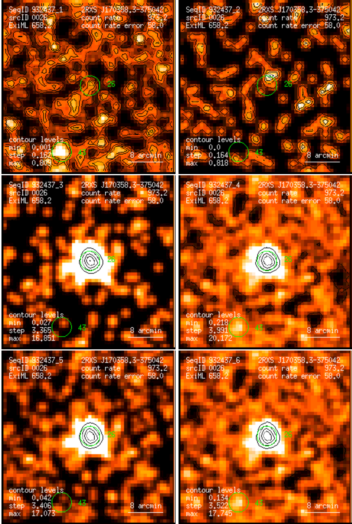
Figure 26: RASS 932437: detection 0026: band rate images, Gaussian filter: (1) PSPC channels 11 – 41, (2) 52 – 90, (3) 91 – 201, (4) 11 – 235, (5) 52 – 201, (6) 11 – 201. Broad band rates in counts/ks. Band rate contour levels in counts/ks/arcmin 2 .
