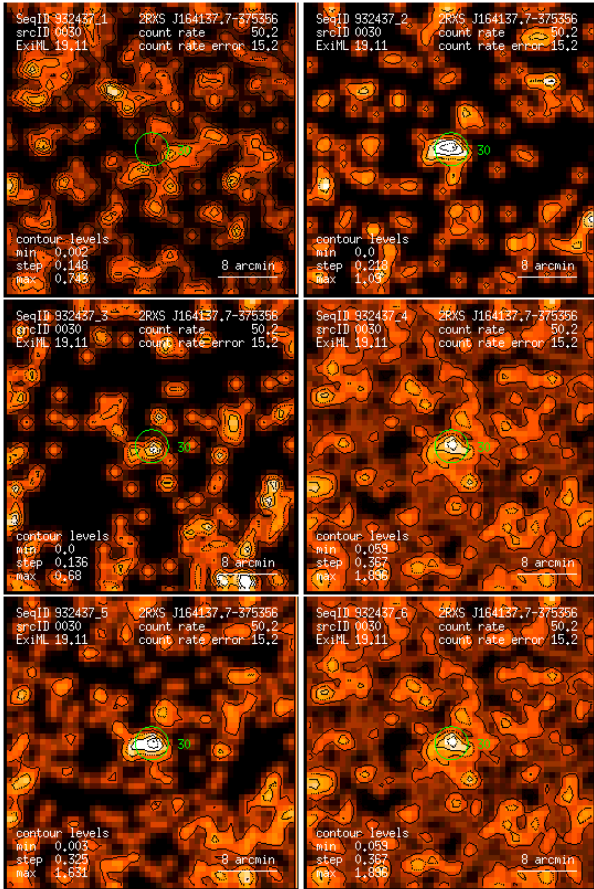
Figure 30: RASS 932437: detection 0030: band rate images, Gaussian filter: (1) PSPC channels 11 – 41, (2) 52 – 90, (3) 91 – 201, (4) 11 – 235, (5) 52 – 201, (6) 11 – 201. Broad band rates in counts/ks. Band rate contour levels in counts/ks/arcmin 2 .
