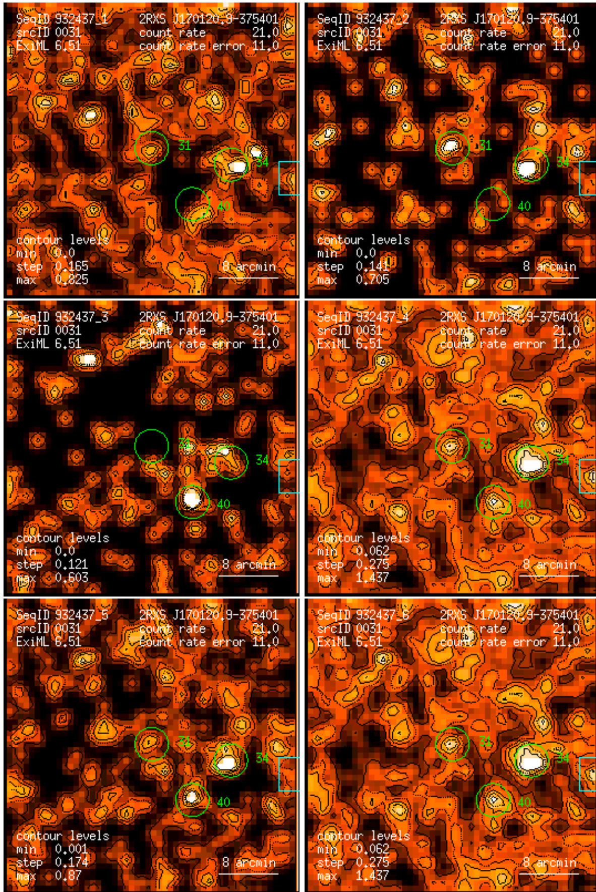
Figure 31: RASS 932437: detection 0031: band rate images, Gaussian filter: (1) PSPC channels 11 – 41, (2) 52 – 90, (3) 91 – 201, (4) 11 – 235, (5) 52 – 201, (6) 11 – 201. Broad band rates in counts/ks. Band rate contour levels in counts/ks/arcmin 2 .
