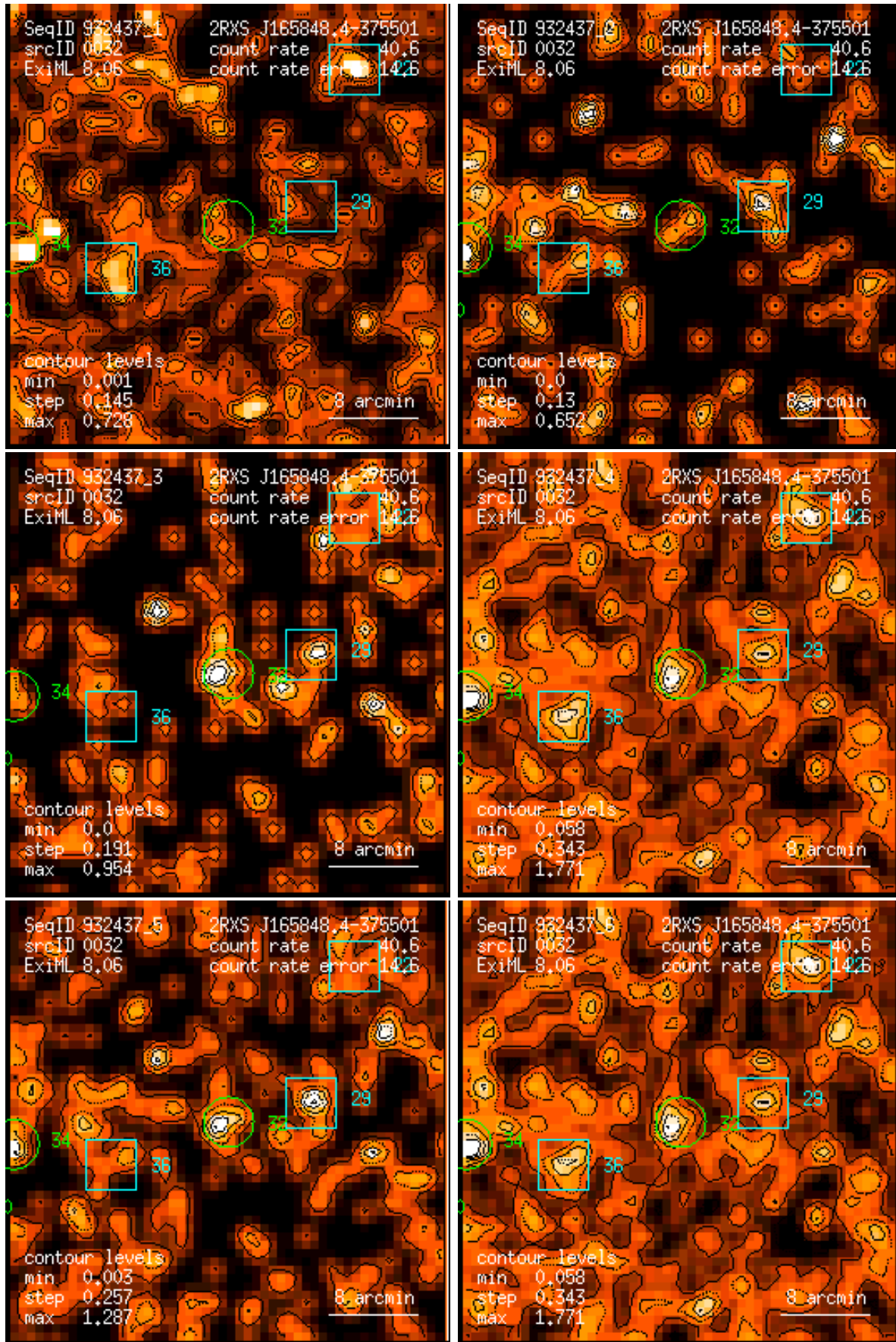
Figure 32: RASS 932437: detection 0032: band rate images, Gaussian filter: (1) PSPC channels 11 – 41, (2) 52 – 90, (3) 91 – 201, (4) 11 – 235, (5) 52 – 201, (6) 11 – 201. Broad band rates in counts/ks. Band rate contour levels in counts/ks/arcmin 2 .
