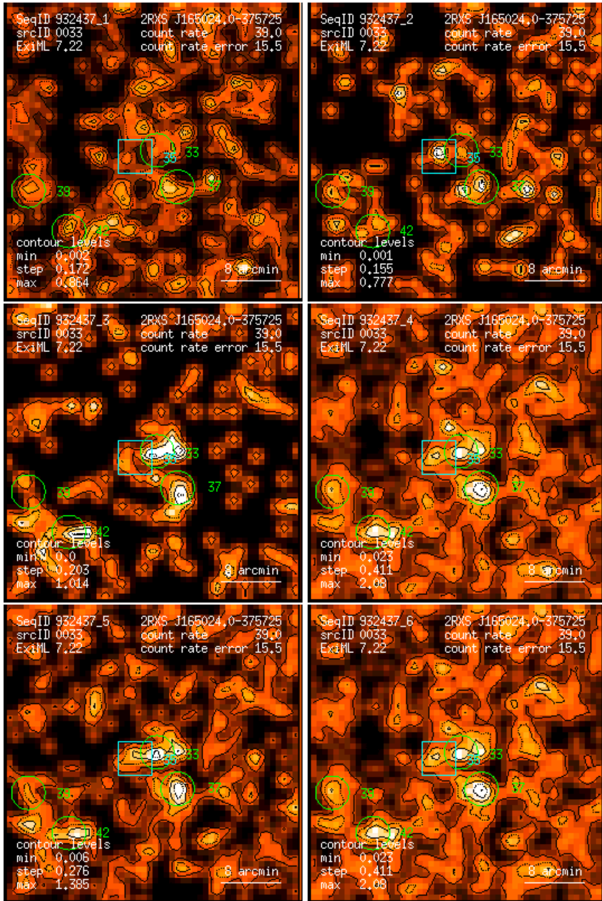
Figure 33: RASS 932437: detection 0033: band rate images, Gaussian filter: (1) PSPC channels 11 – 41, (2) 52 – 90, (3) 91 – 201, (4) 11 – 235, (5) 52 – 201, (6) 11 – 201. Broad band rates in counts/ks. Band rate contour levels in counts/ks/arcmin 2 .
