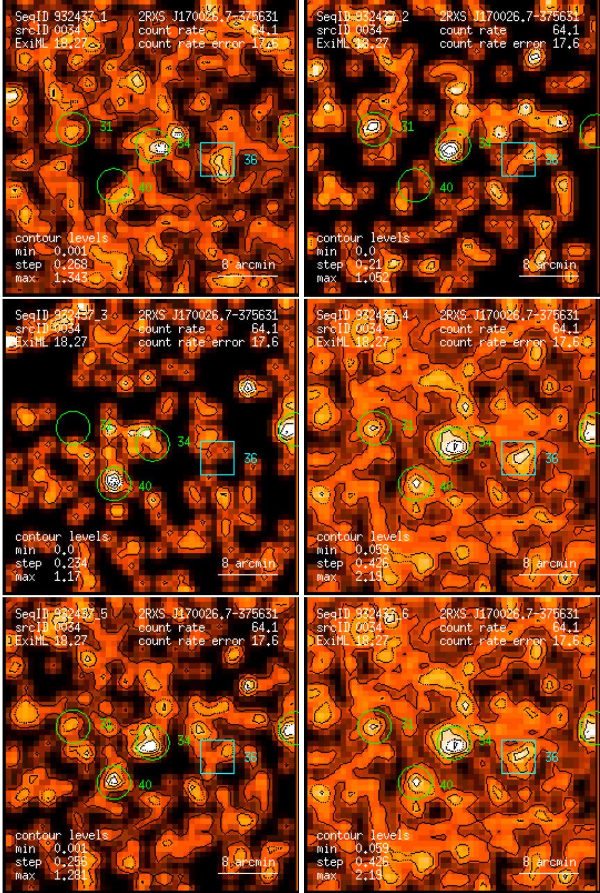
Figure 34: RASS 932437: detection 0034: band rate images, Gaussian filter: (1) PSPC channels 11 – 41, (2) 52 – 90, (3) 91 – 201, (4) 11 – 235, (5) 52 – 201, (6) 11 – 201. Broad band rates in counts/ks. Band rate contour levels in counts/ks/arcmin 2 .
