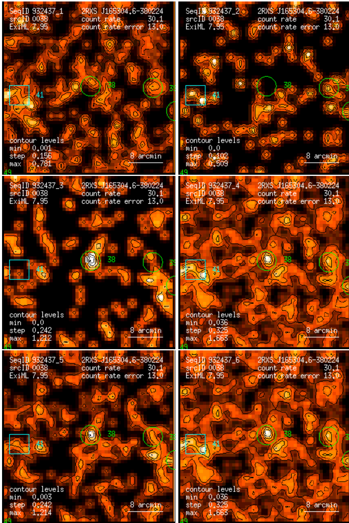
Figure 38: RASS 932437: detection 0038: band rate images, Gaussian filter: (1) PSPC channels 11 – 41, (2) 52 – 90, (3) 91 – 201, (4) 11 – 235, (5) 52 – 201, (6) 11 – 201. Broad band rates in counts/ks. Band rate contour levels in counts/ks/arcmin 2 .
