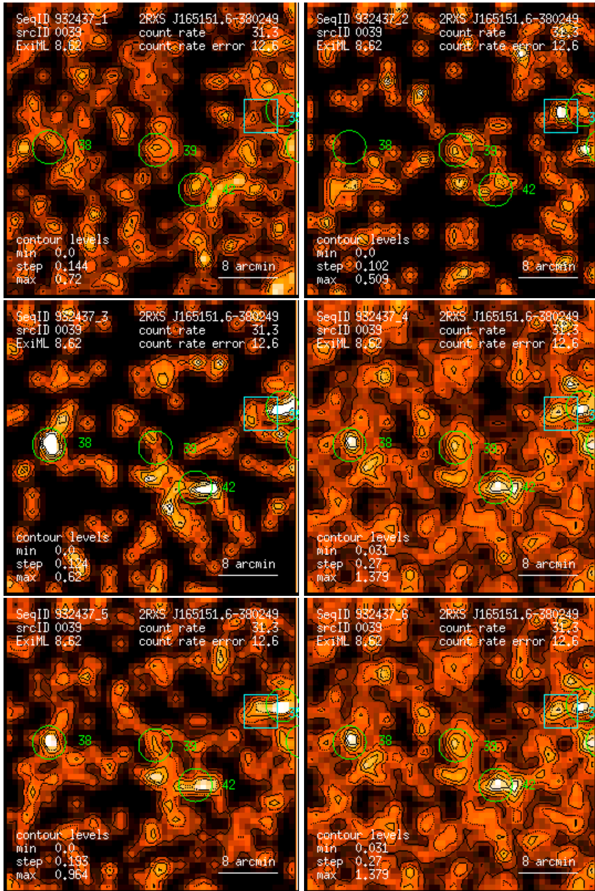
Figure 39: RASS 932437: detection 0039: band rate images, Gaussian filter: (1) PSPC channels 11 – 41, (2) 52 – 90, (3) 91 – 201, (4) 11 – 235, (5) 52 – 201, (6) 11 – 201. Broad band rates in counts/ks. Band rate contour levels in counts/ks/arcmin 2 .
