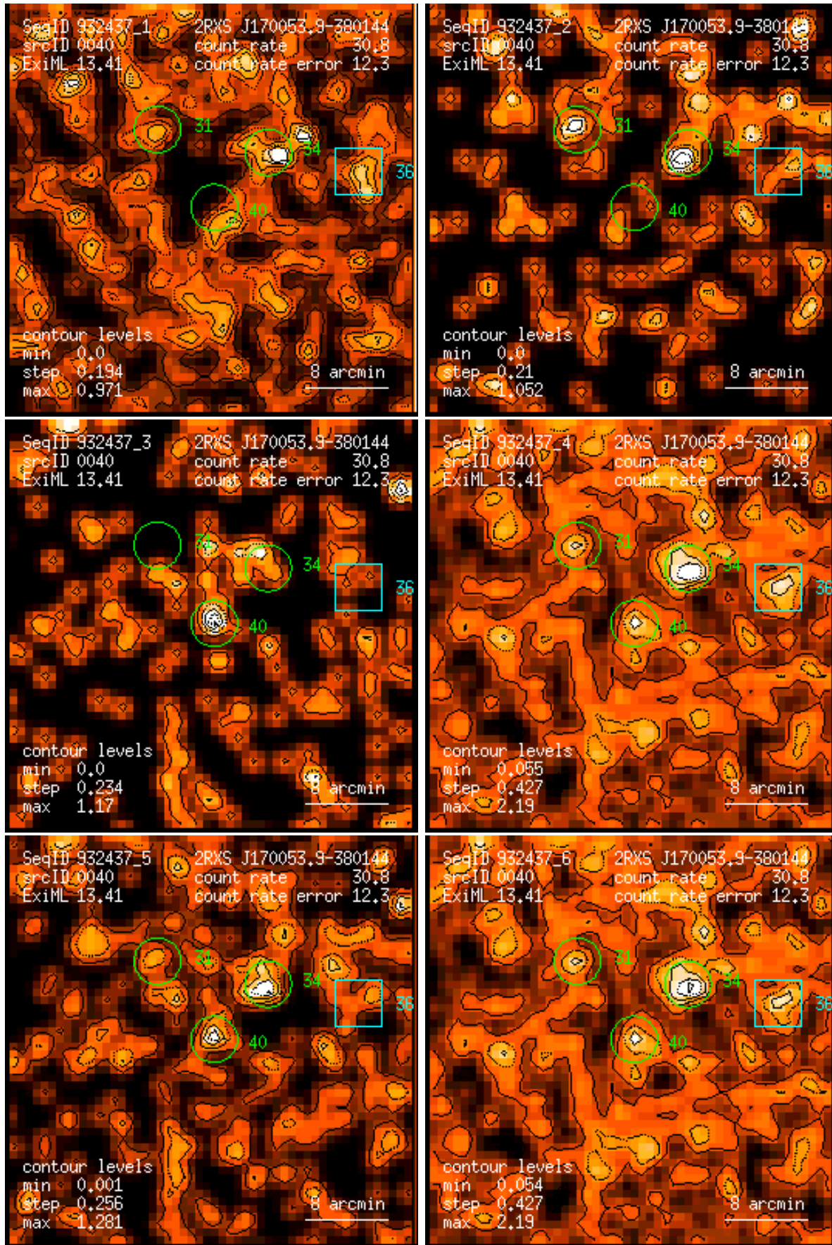
Figure 40: RASS 932437: detection 0040: band rate images, Gaussian filter: (1) PSPC channels 11 – 41, (2) 52 – 90, (3) 91 – 201, (4) 11 – 235, (5) 52 – 201, (6) 11 – 201. Broad band rates in counts/ks. Band rate contour levels in counts/ks/arcmin 2 .
