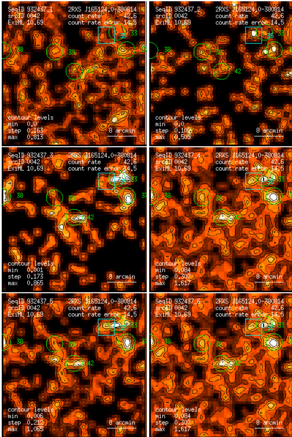
Figure 42: RASS 932437: detection 0042: band rate images, Gaussian filter: (1) PSPC channels 11 – 41, (2) 52 – 90, (3) 91 – 201, (4) 11 – 235, (5) 52 – 201, (6) 11 – 201. Broad band rates in counts/ks. Band rate contour levels in counts/ks/arcmin 2 .
