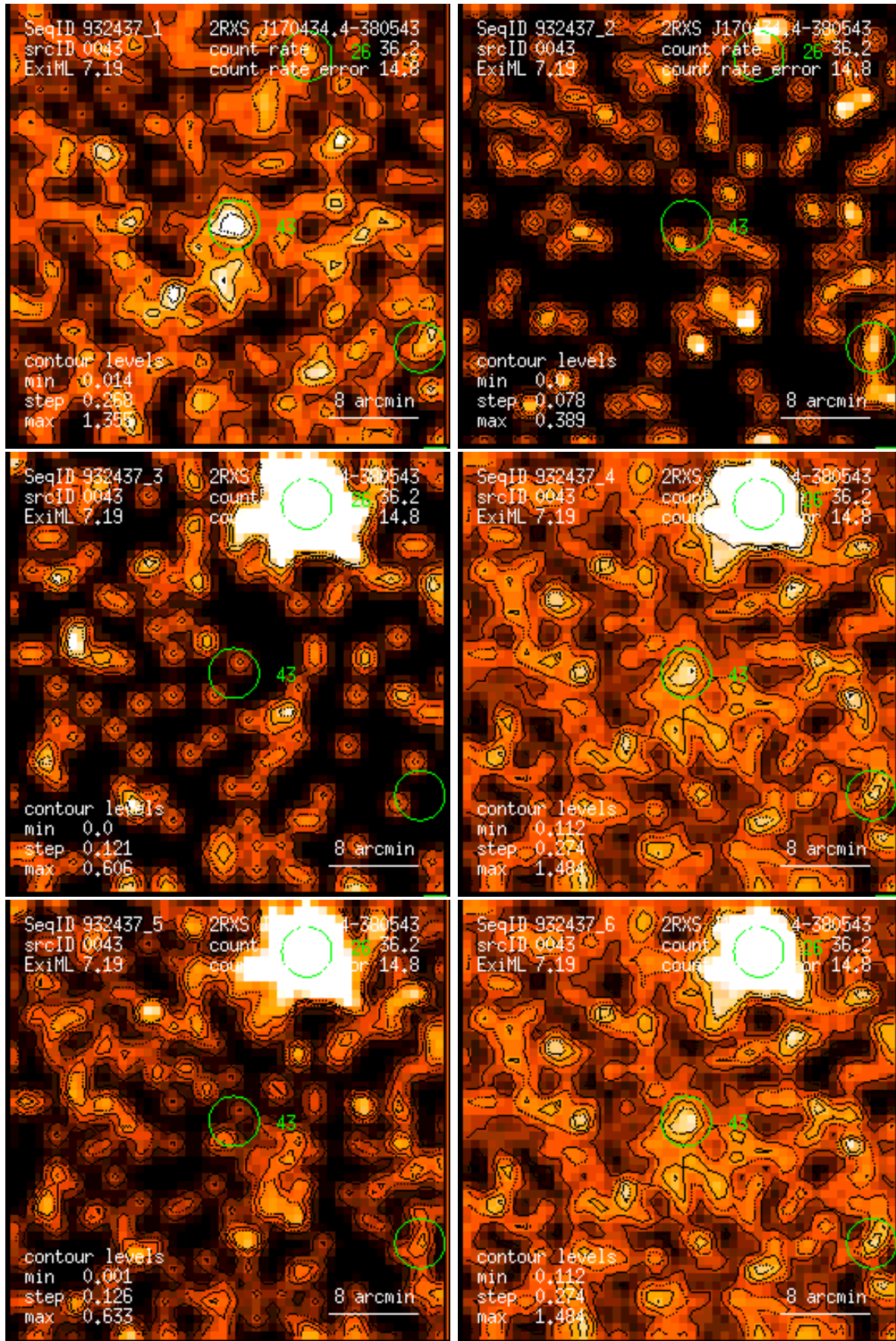
Figure 43: RASS 932437: detection 0043: band rate images, Gaussian filter: (1) PSPC channels 11 – 41, (2) 52 – 90, (3) 91 – 201, (4) 11 – 235, (5) 52 – 201, (6) 11 – 201. Broad band rates in counts/ks. Band rate contour levels in counts/ks/arcmin 2 .
