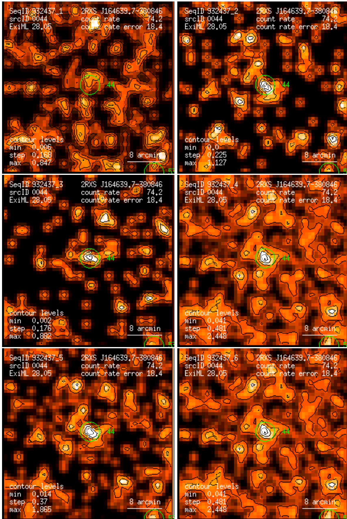
Figure 44: RASS 932437: detection 0044: band rate images, Gaussian filter: (1) PSPC channels 11 – 41, (2) 52 – 90, (3) 91 – 201, (4) 11 – 235, (5) 52 – 201, (6) 11 – 201. Broad band rates in counts/ks. Band rate contour levels in counts/ks/arcmin 2 .
