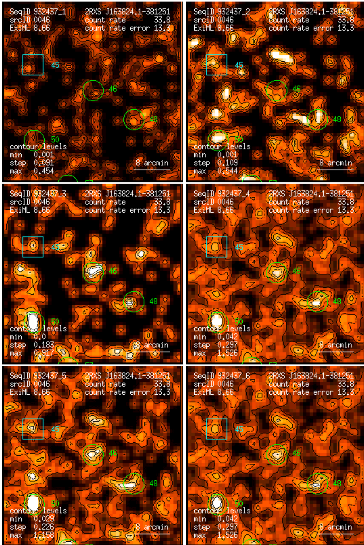
Figure 46: RASS 932437: detection 0046: band rate images, Gaussian filter: (1) PSPC channels 11 – 41, (2) 52 – 90, (3) 91 – 201, (4) 11 – 235, (5) 52 – 201, (6) 11 – 201. Broad band rates in counts/ks. Band rate contour levels in counts/ks/arcmin 2 .
