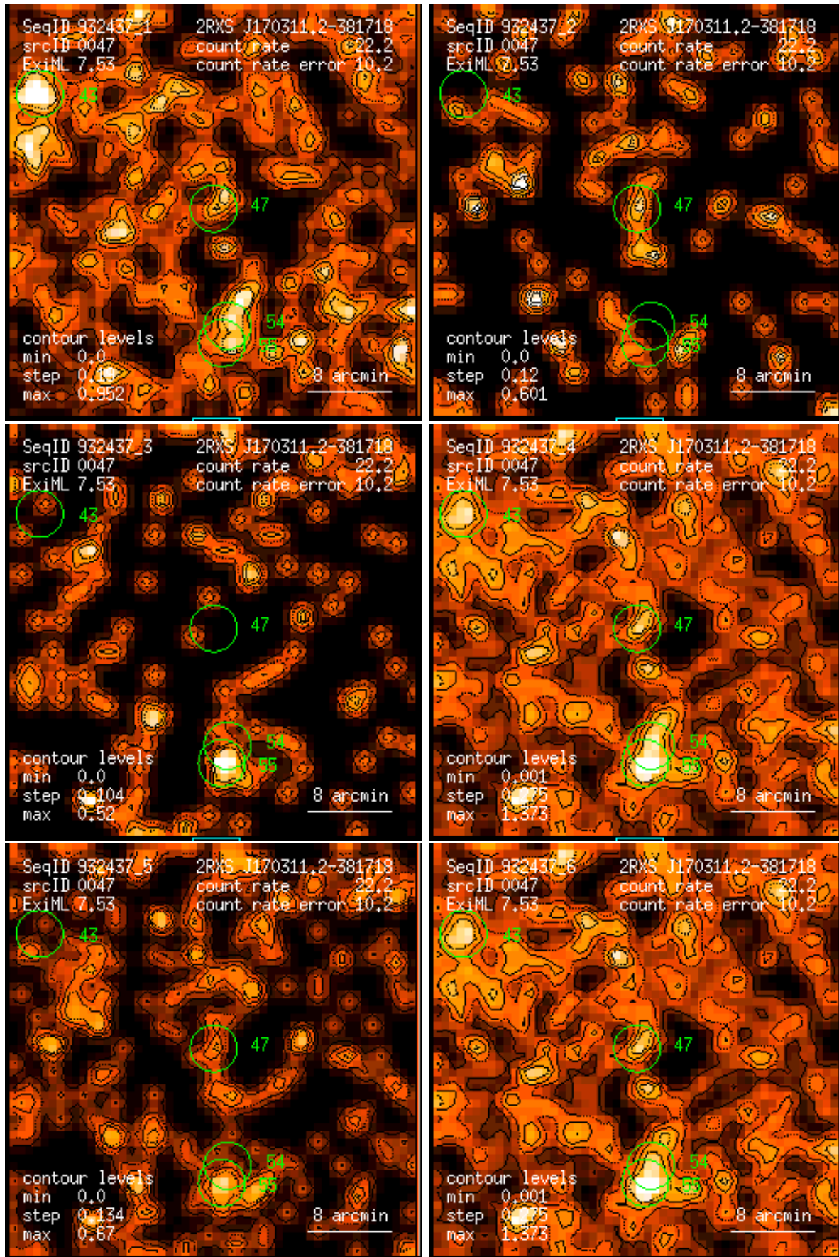
Figure 47: RASS 932437: detection 0047: band rate images, Gaussian filter: (1) PSPC channels 11 – 41, (2) 52 – 90, (3) 91 – 201, (4) 11 – 235, (5) 52 – 201, (6) 11 – 201. Broad band rates in counts/ks. Band rate contour levels in counts/ks/arcmin 2 .
