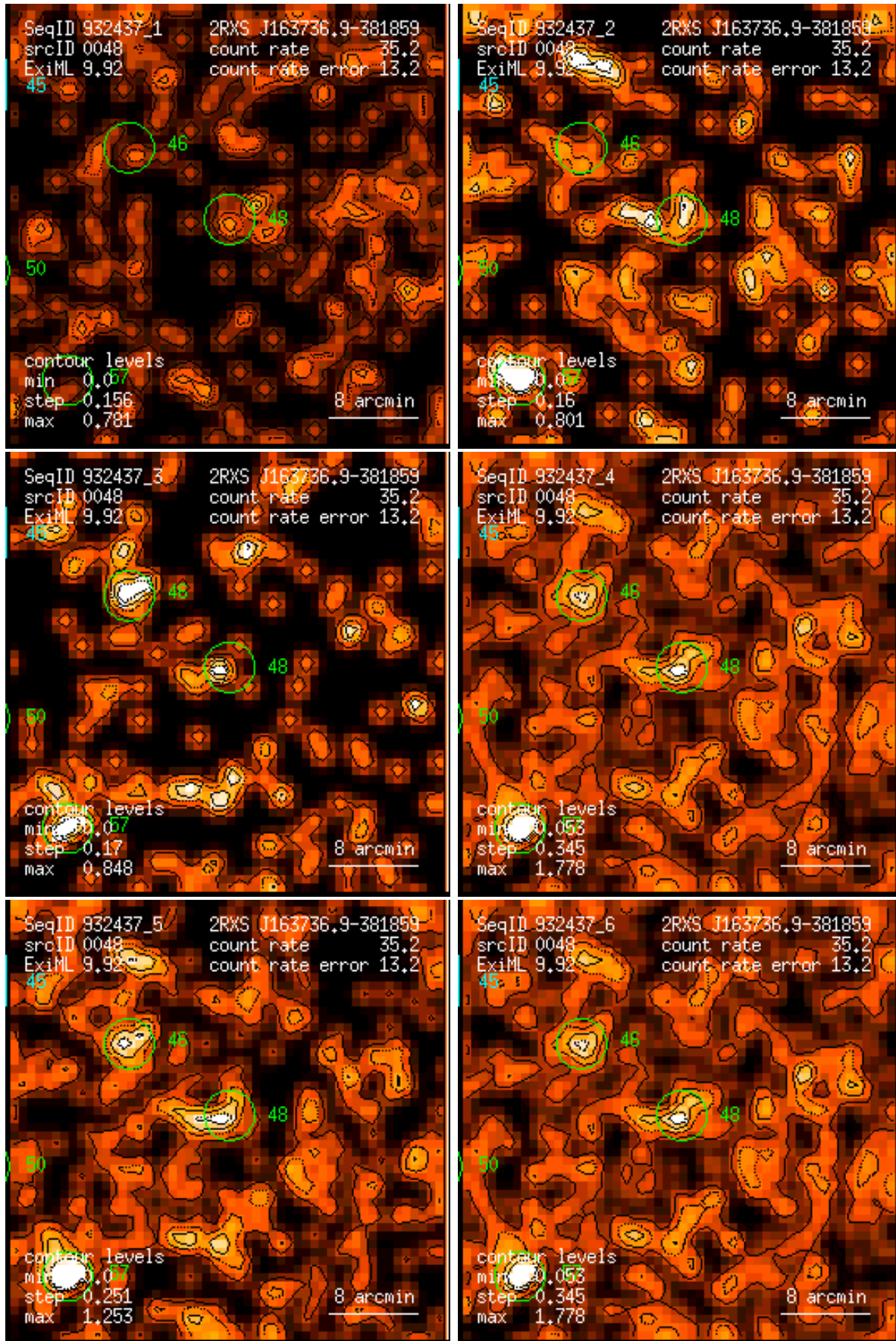
Figure 48: RASS 932437: detection 0048: band rate images, Gaussian filter: (1) PSPC channels 11 – 41, (2) 52 – 90, (3) 91 – 201, (4) 11 – 235, (5) 52 – 201, (6) 11 – 201. Broad band rates in counts/ks. Band rate contour levels in counts/ks/arcmin 2 .
