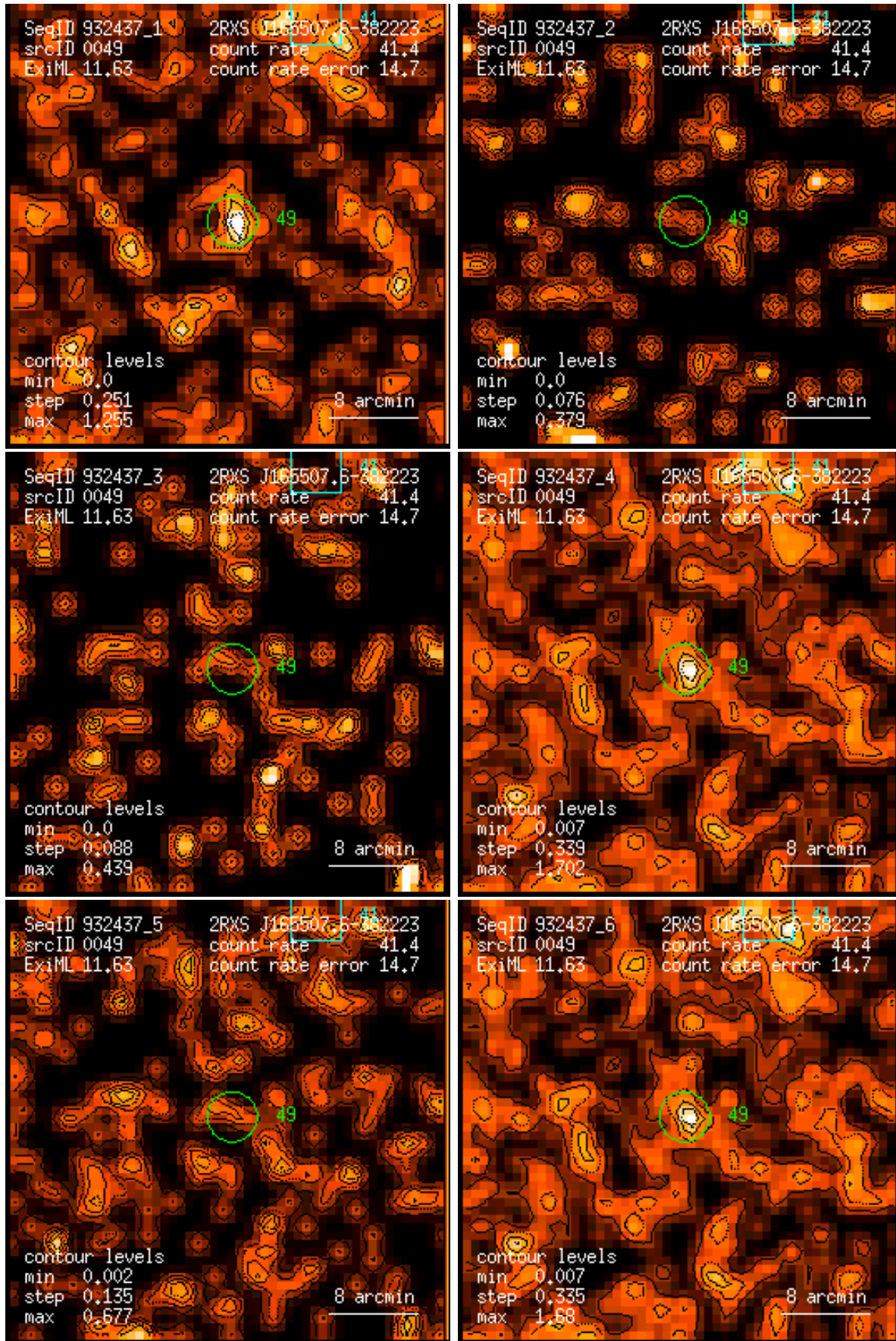
Figure 49: RASS 932437: detection 0049: band rate images, Gaussian filter: (1) PSPC channels 11 – 41, (2) 52 – 90, (3) 91 – 201, (4) 11 – 235, (5) 52 – 201, (6) 11 – 201. Broad band rates in counts/ks. Band rate contour levels in counts/ks/arcmin 2 .
