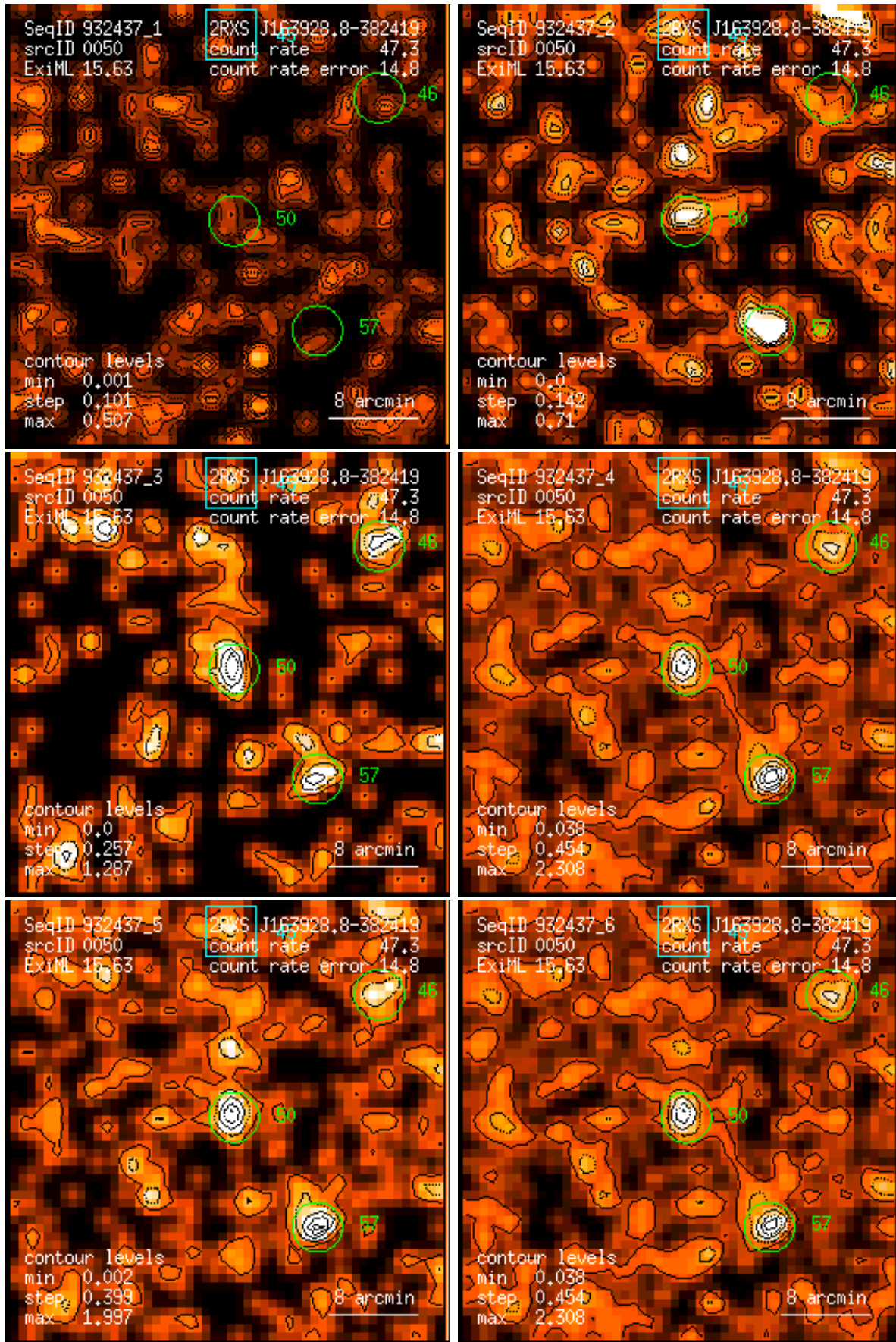
Figure 50: RASS 932437: detection 0050: band rate images, Gaussian filter: (1) PSPC channels 11 – 41, (2) 52 – 90, (3) 91 – 201, (4) 11 – 235, (5) 52 – 201, (6) 11 – 201. Broad band rates in counts/ks. Band rate contour levels in counts/ks/arcmin 2 .
