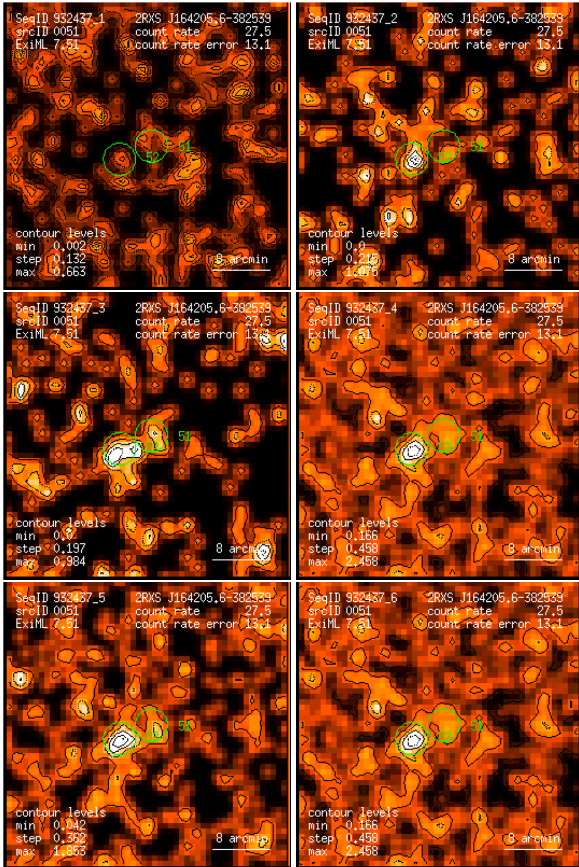
Figure 51: RASS 932437: detection 0051: band rate images, Gaussian filter: (1) PSPC channels 11 – 41, (2) 52 – 90, (3) 91 – 201, (4) 11 – 235, (5) 52 – 201, (6) 11 – 201. Broad band rates in counts/ks. Band rate contour levels in counts/ks/arcmin 2 .
