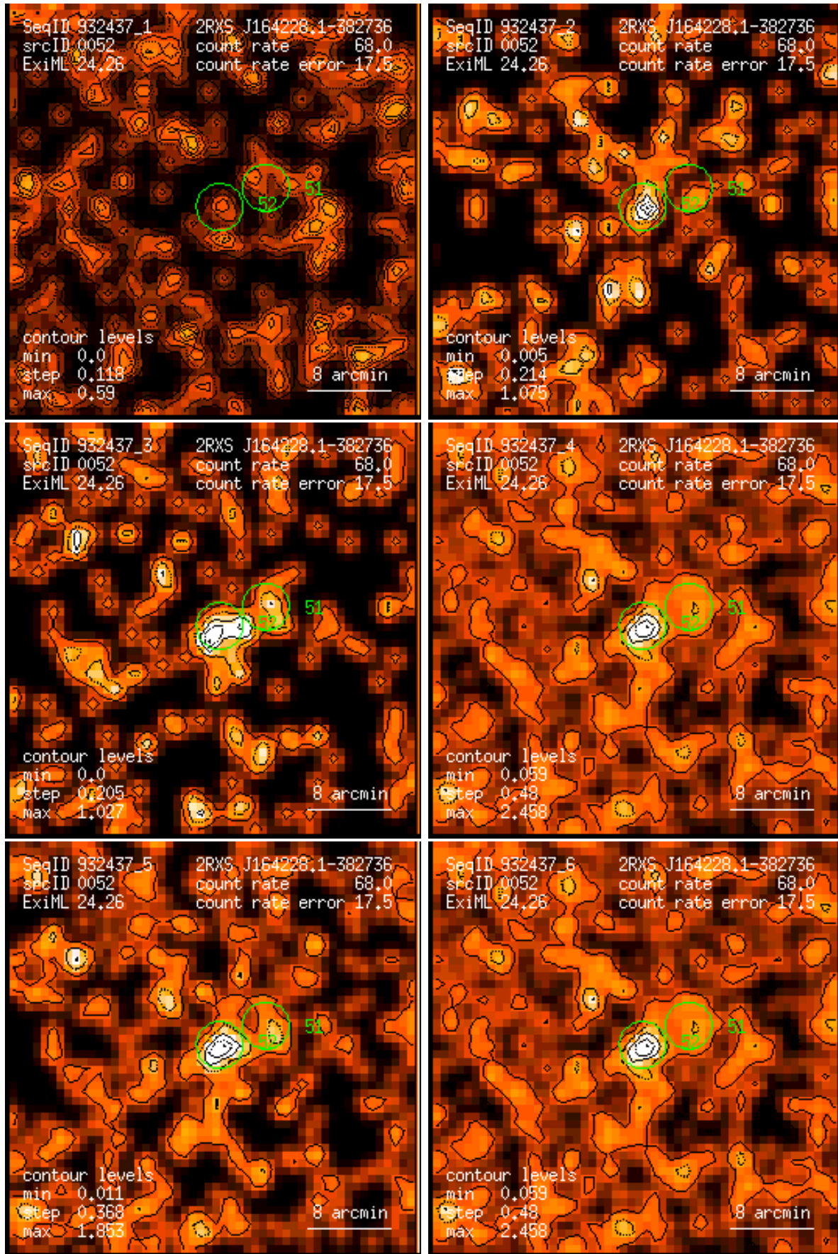
Figure 52: RASS 932437: detection 0052: band rate images, Gaussian filter: (1) PSPC channels 11 – 41, (2) 52 – 90, (3) 91 – 201, (4) 11 – 235, (5) 52 – 201, (6) 11 – 201. Broad band rates in counts/ks. Band rate contour levels in counts/ks/arcmin 2 .
