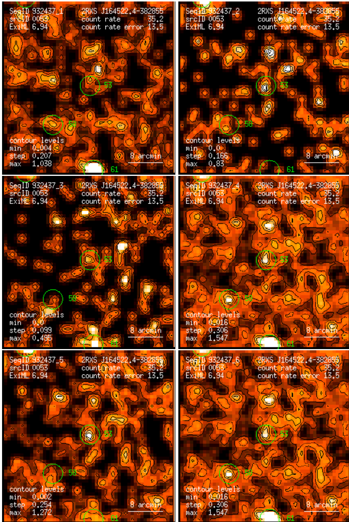
Figure 53: RASS 932437: detection 0053: band rate images, Gaussian filter: (1) PSPC channels 11 – 41, (2) 52 – 90, (3) 91 – 201, (4) 11 – 235, (5) 52 – 201, (6) 11 – 201. Broad band rates in counts/ks. Band rate contour levels in counts/ks/arcmin 2 .
